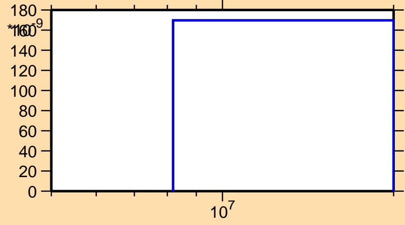
\sigma vs. E for ^{210}\text{Pb}(n,\text{nt})
