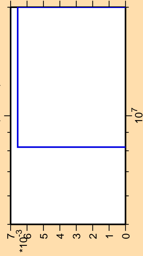
\Delta\sigma/\sigma vs. E for ^{210}\text{Pb}(n,3n\alpha)
