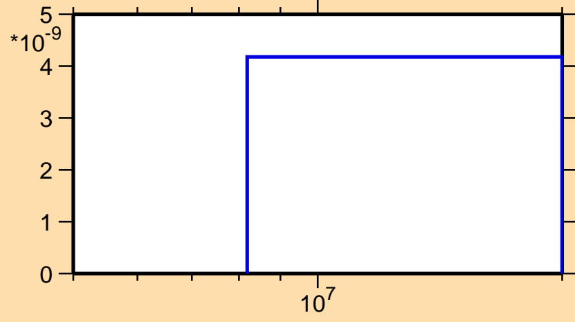
\sigma vs. E for ^{210}\text{Pb}(n,\text{nd})
