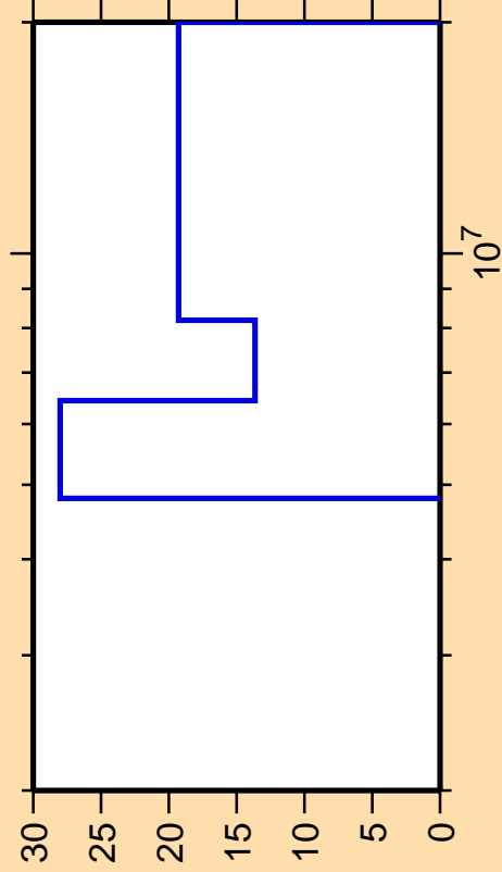
\Delta\sigma/\sigma vs. E for ^{210}\text{Pb}(n,2n)
