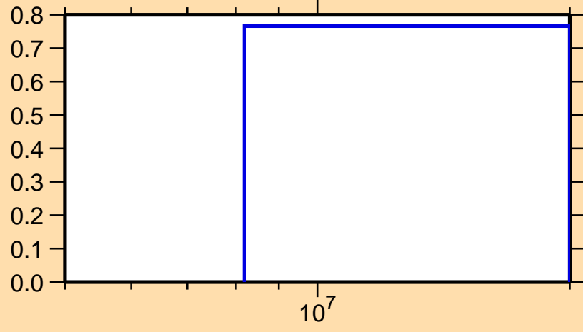
\sigma vs. E for ^{210}\text{Pb}(n,3n)
