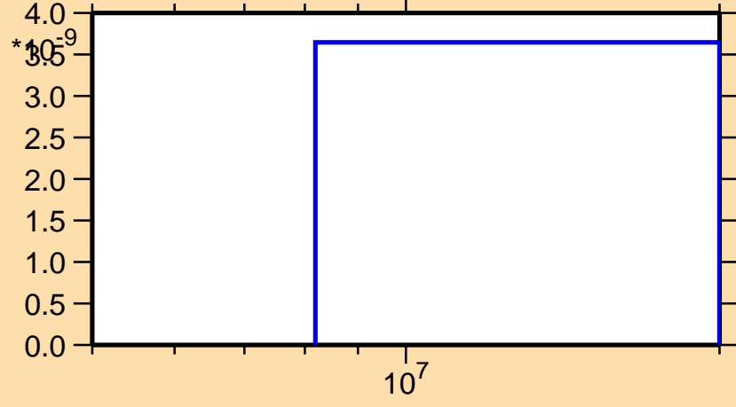
\sigma vs. E for ^{210}\text{Pb}(n,2n\alpha)
