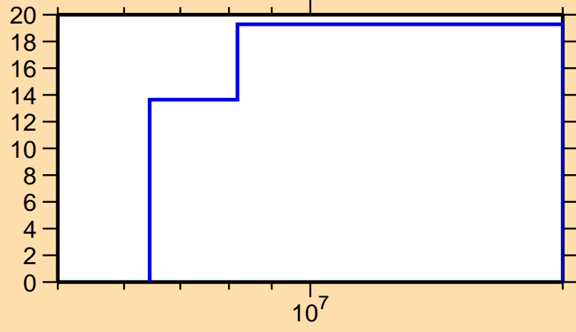
\Delta\sigma/\sigma vs. E for ^{210}\text{Pb}(n,2n)
