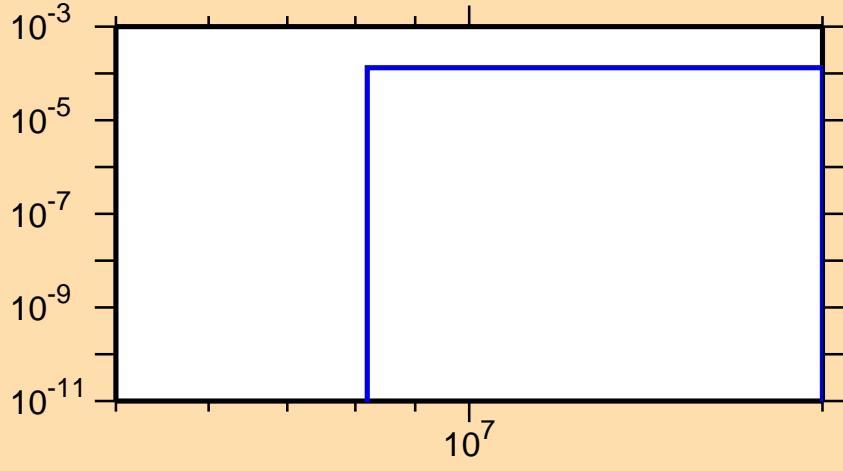
\sigma vs. E for ^{210}\text{Pb}(n,p)
