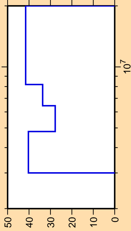
\Delta\sigma/\sigma vs. E for ^{210}\text{Pb}(n,n\text{cont.})
