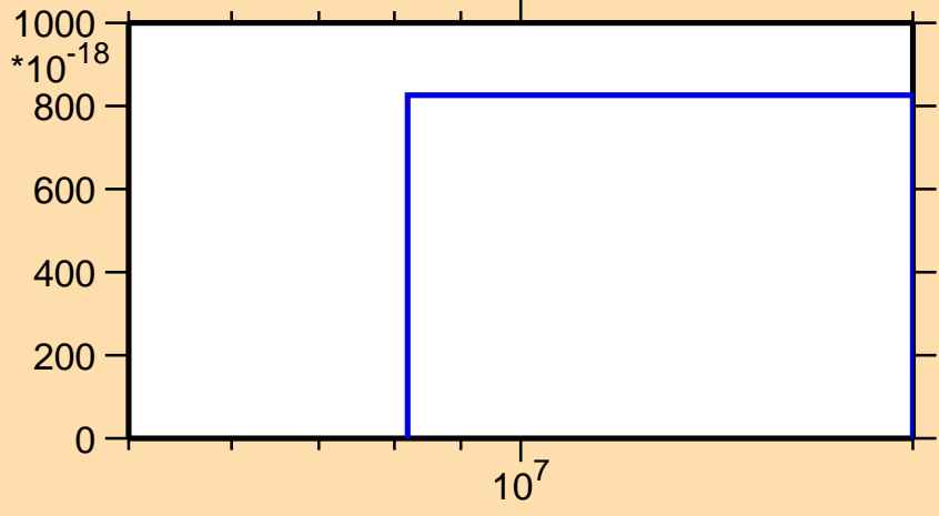
\sigma vs. E for ^{210}\text{Pb}(n,3n\alpha)
