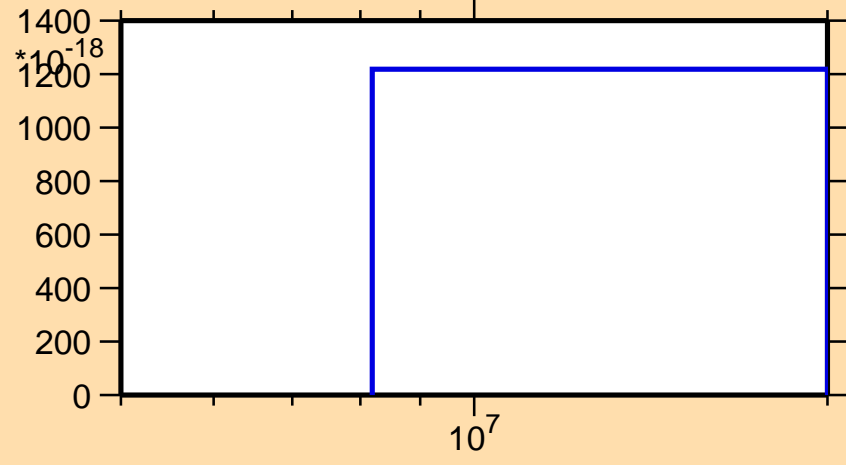
\sigma vs. E for ^{210}\text{Pb} (mt 11)
