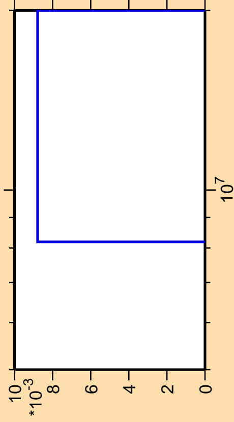
\Delta\sigma/\sigma vs. E for ^{210}\text{Pb} (mt 11)
