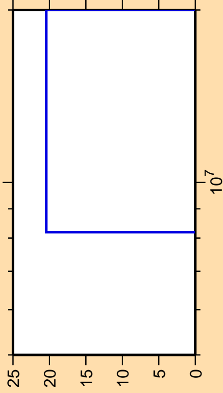
\Delta\sigma/\sigma vs. E for ^{210}\text{Pb}(n,3n)
