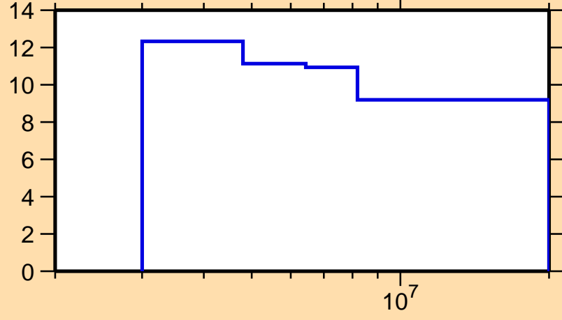
\Delta\sigma/\sigma vs. E for ^{210}\text{Pb}(n,n\text{nonel.})
