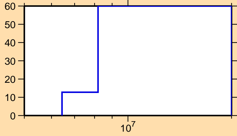
\Delta\sigma/\sigma vs. E for ^{210}\text{Pb}(n,p)
