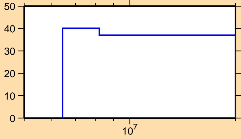
\Delta\sigma/\sigma vs. E for ^{210}\text{Pb}(n,n_1)
