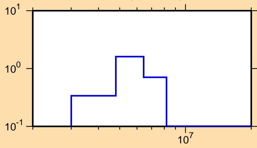
\sigma vs. E for ^{210}\text{Pb}(n,n\text{cont.})
