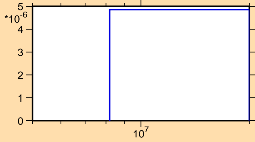
\sigma vs. E for ^{210}\text{Pb}(n,np)
