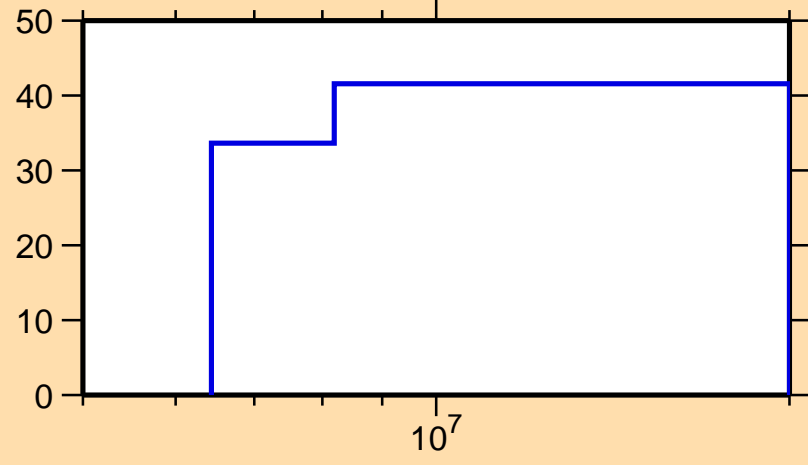
\Delta\sigma/\sigma vs. E for ^{210}\text{Pb}(n,ncont.)
