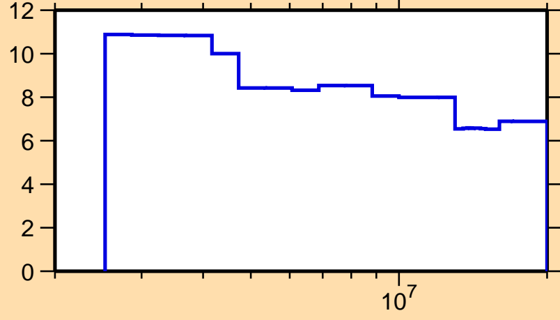
\Delta\sigma/\sigma vs. E for ^{211}\text{Pb}(n,n\text{nonel.})
