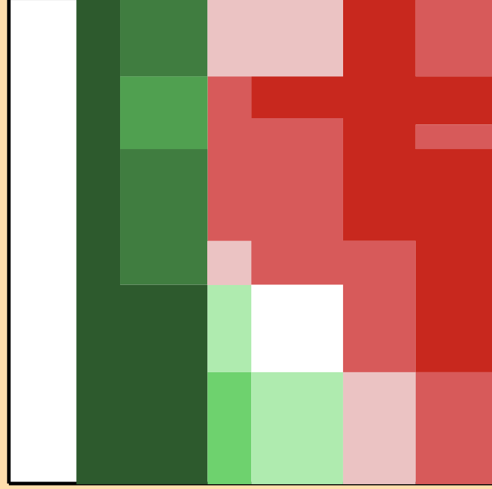
\Delta\sigma/\sigma vs. E for ^{211}\text{Pb}(n,p)
