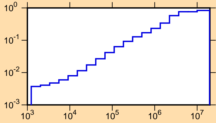
\mu vs. E for ^{211}\text{Pb}(\text{mt251})
