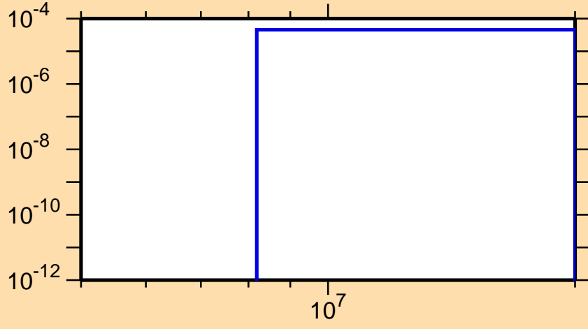
\sigma vs. E for ^{211}\text{Pb}(n,t)
