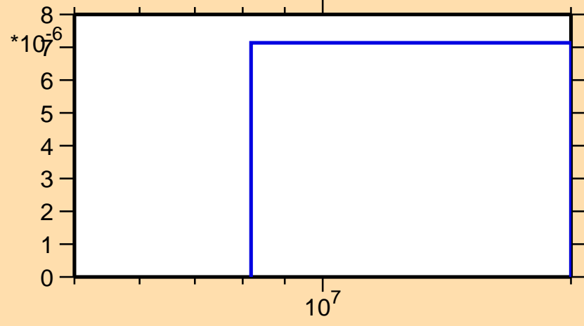
\sigma vs. E for ^{211}\text{Pb}(n,np)
