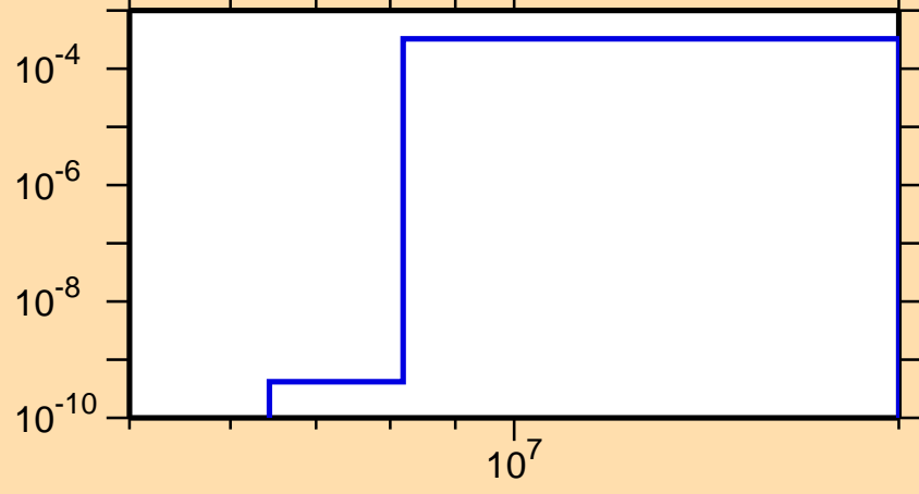
\sigma vs. E for ^{211}\text{Pb}(n,p)
