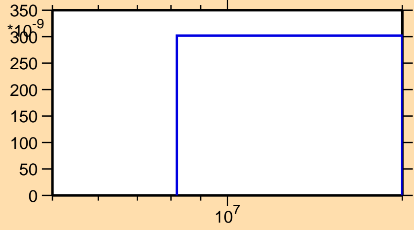
\sigma vs. E for ^{211}\text{Pb}(n,\text{nt})
