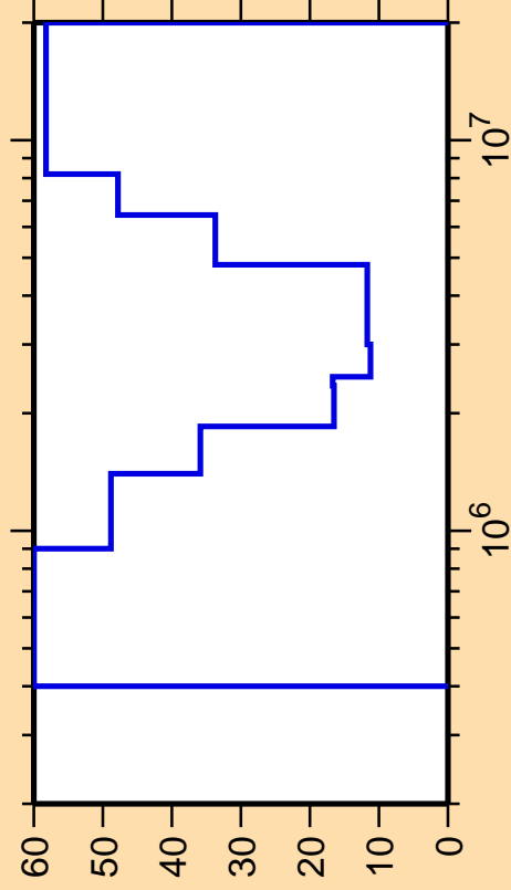
\Delta\sigma/\sigma vs. E for ^{211}\text{Pb}(n,\text{inel.})
