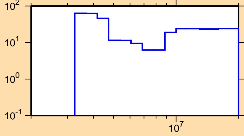
\Delta\sigma/\sigma vs. E for ^{215}\text{Pb}(n,2n)
