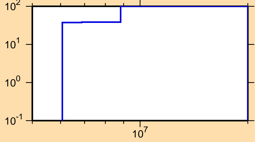
\Delta\sigma/\sigma vs. E for ^{219}\text{Pb}(n,\gamma)
