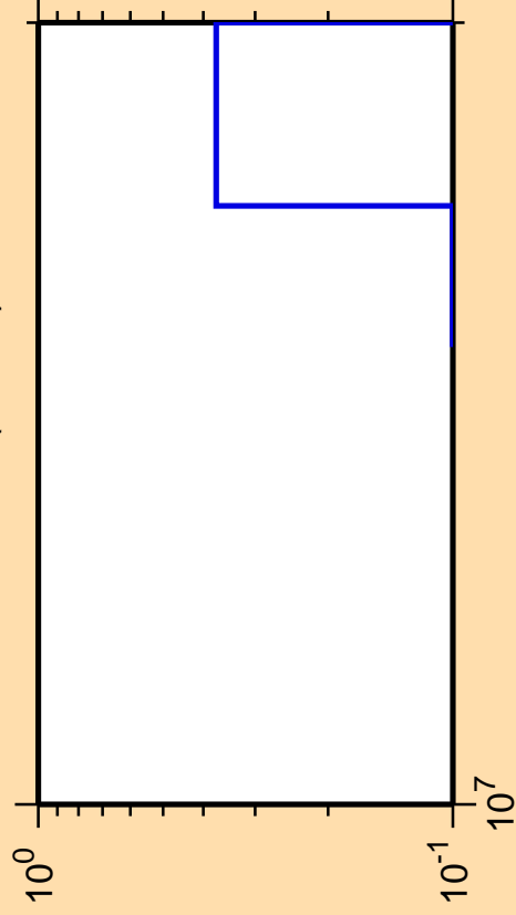
\Delta\sigma/\sigma vs. E for ^{219}\text{Pb}(\text{mt } 11)
