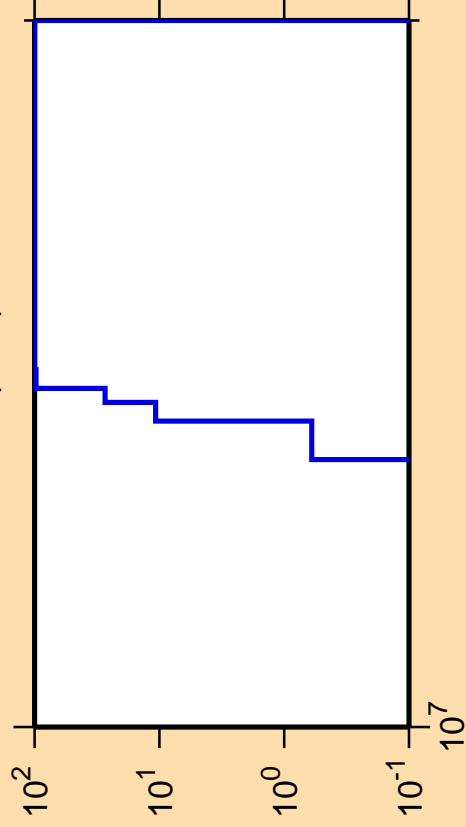
\Delta\sigma/\sigma vs. E for ^{219}\text{Pb}(n,\text{nt})
