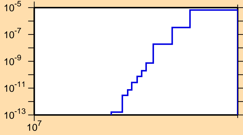
\sigma vs. E for ^{219}\text{Pb}(n,\text{nt})
