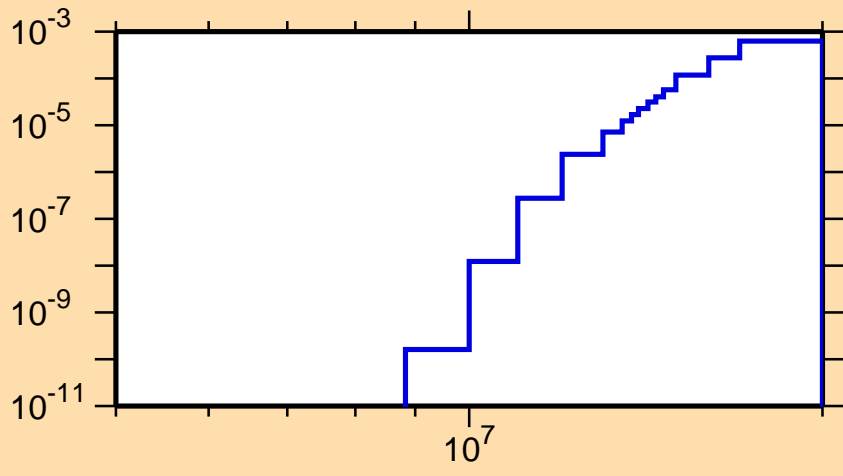
\sigma vs. E for ^{219}\text{Pb}(n,p)
