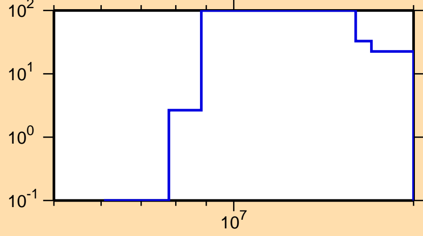
\Delta\sigma/\sigma vs. E for ^{219}\text{Pb}(n,p)
