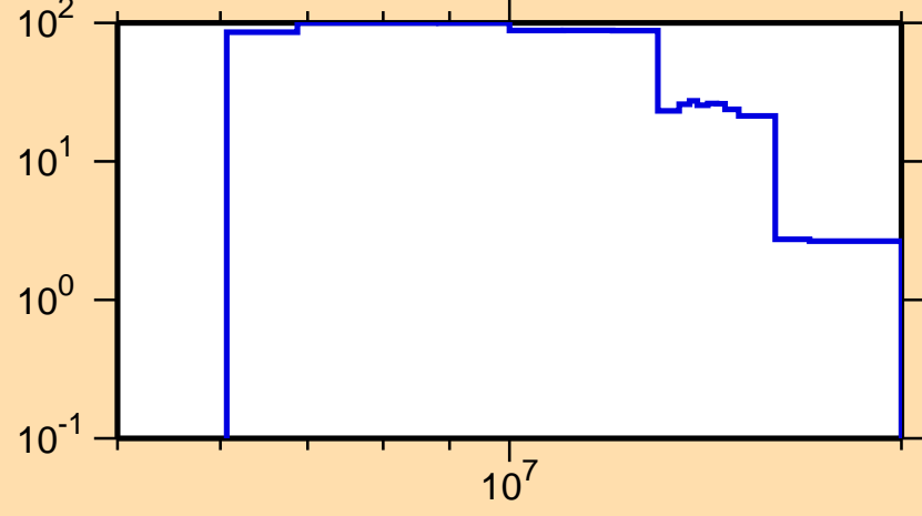
\Delta\sigma/\sigma vs. E for ^{219}\text{Pb}(n,\text{el.})
