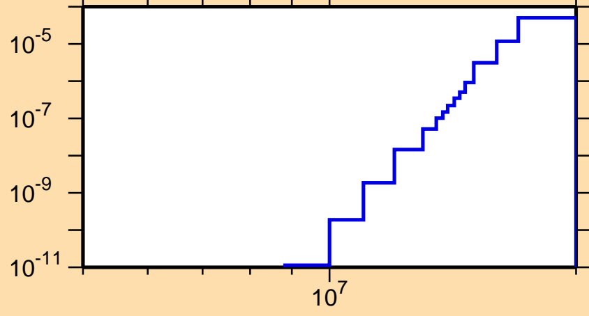
\sigma vs. E for ^{219}\text{Pb}(n,n\alpha)
