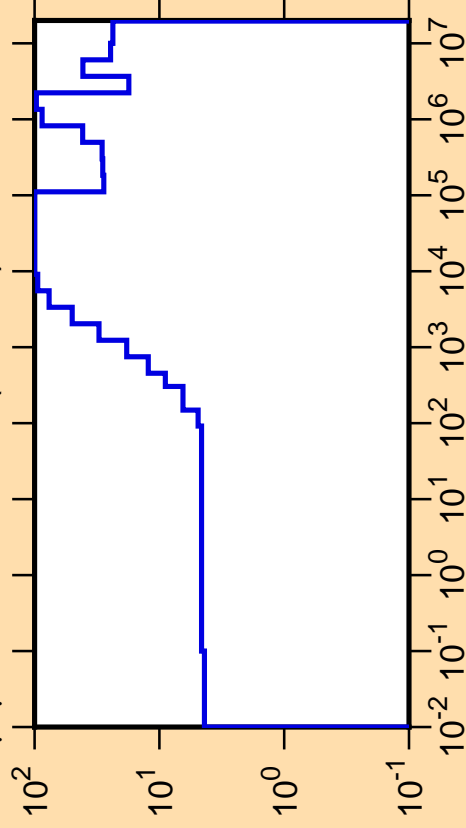
\Delta\mu/\mu vs. E for ^{219}\text{Pb}(\text{mt251})
