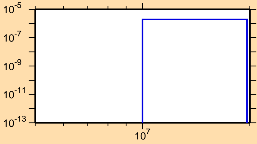
\sigma vs. E for ^{219}\text{Pb}(n,d)
