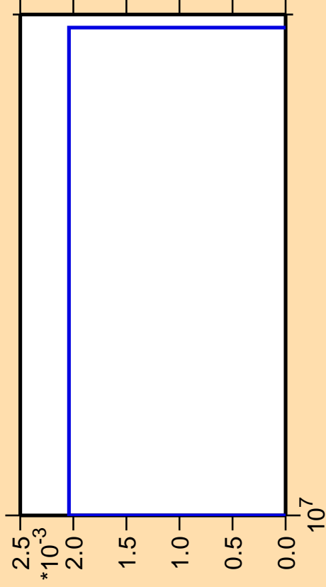
\Delta\sigma/\sigma vs. E for ^{219}\text{Pb}(\text{mt 11})
