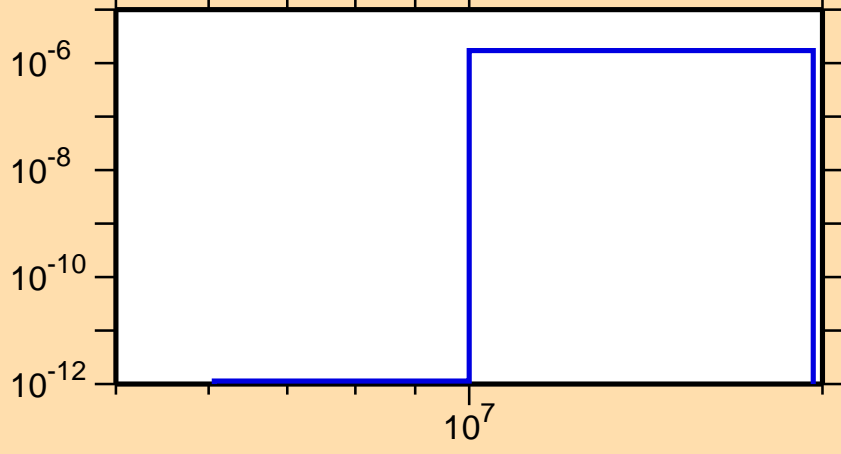
\sigma vs. E for ^{219}\text{Pb}(n,n\alpha)
