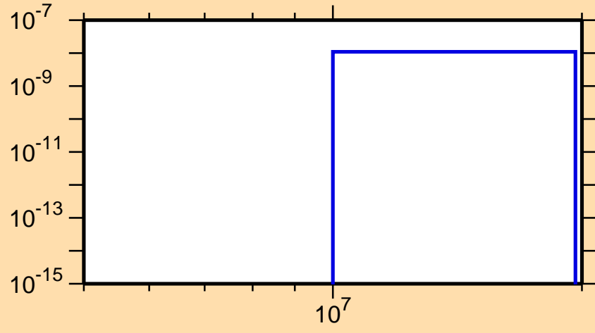
\sigma vs. E for ^{219}\text{Pb}(n,2n\alpha)
