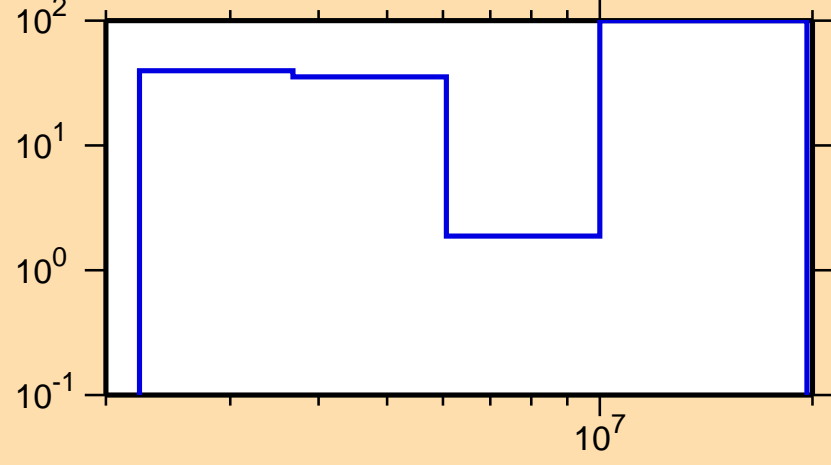
\Delta\sigma/\sigma vs. E for ^{219}\text{Pb}(n,2n)
