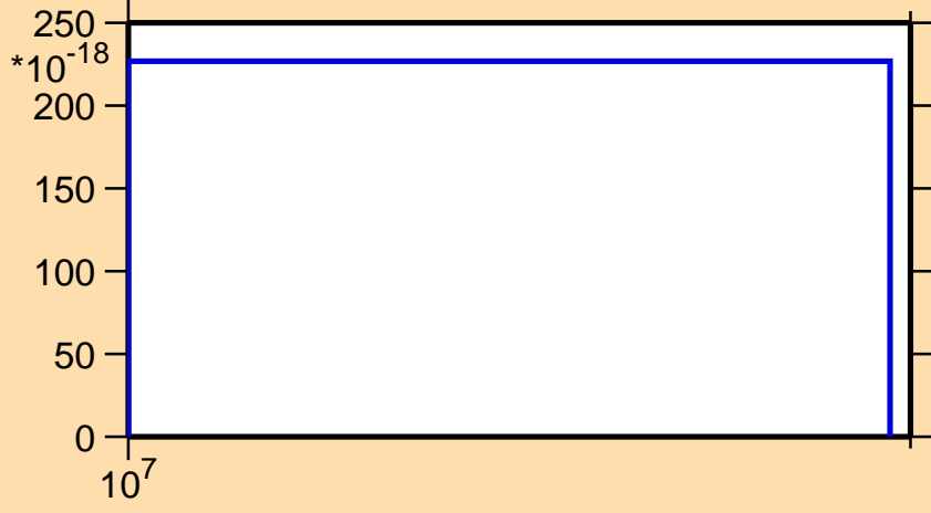
\sigma vs. E for ^{219}\text{Pb}(\text{mt 11})
