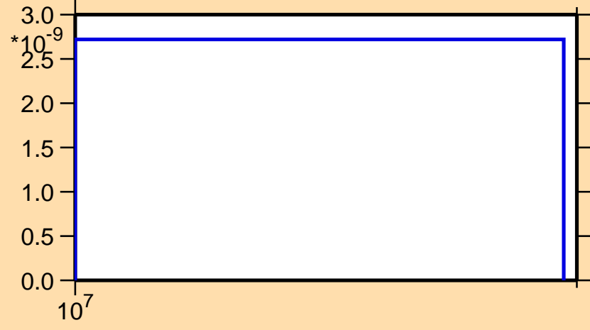
\sigma vs. E for ^{219}\text{Pb}(n,\text{nd})
