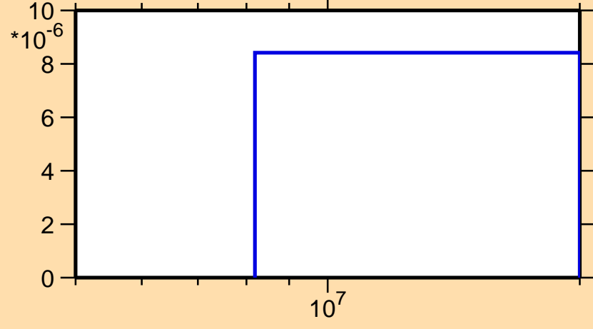
\sigma vs. E for ^{219}\text{Pb}(n,t)
