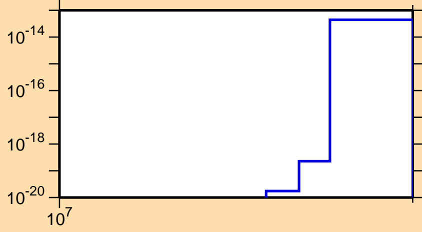
\sigma vs. E for ^{220}\text{Pb}(\text{mt } 11)
