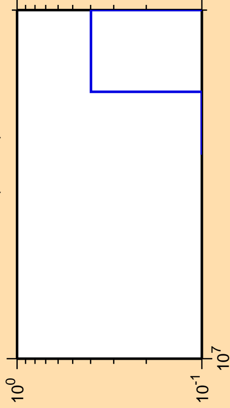
\Delta\sigma/\sigma vs. E for ^{220}\text{Pb}(\text{mt } 11)
