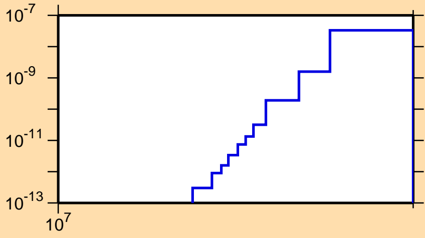
\sigma vs. E for ^{220}\text{Pb}(n,2n\alpha)
