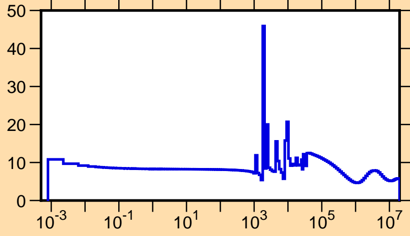
\sigma vs. E for ^{220}\text{Pb}(n,\text{tot.})
