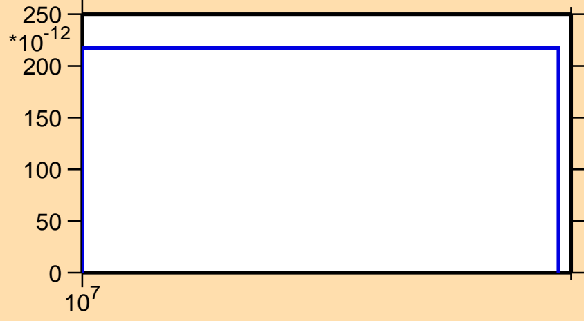
\sigma vs. E for ^{220}\text{Pb}(n,\text{nd})
