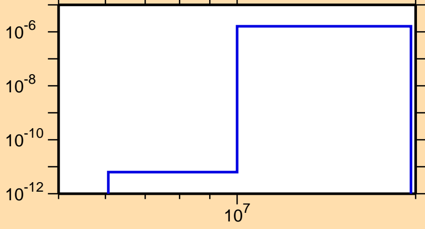
\sigma vs. E for ^{220}\text{Pb}(n,\alpha)
