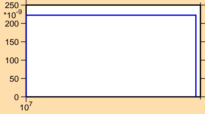
\sigma vs. E for ^{220}\text{Pb}(n,np)
