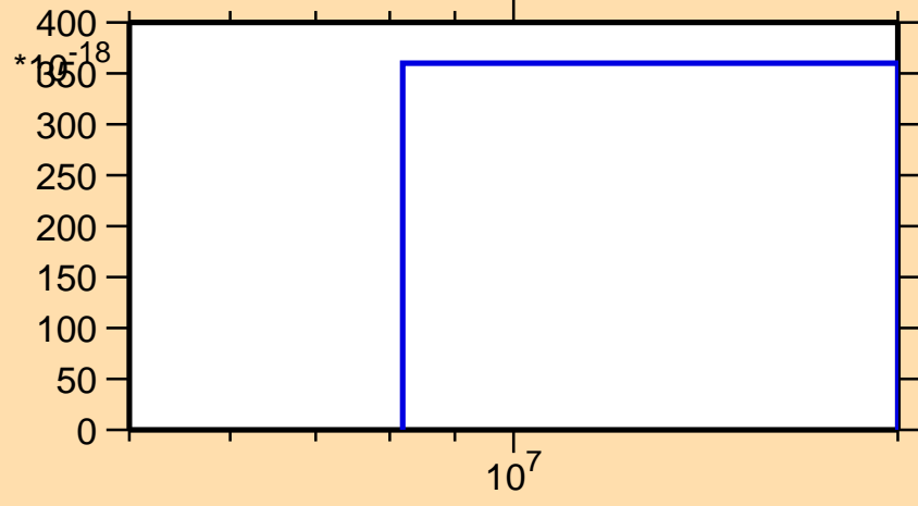
\sigma vs. E for ^{220}\text{Pb} (mt 11)
