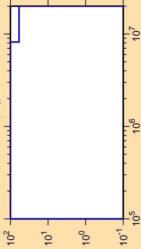
\Delta\sigma/\sigma vs. E for ^{220}\text{Pb}(n,\gamma)
