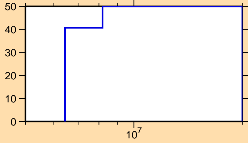
\Delta\sigma/\sigma vs. E for ^{220}\text{Pb}(n,\text{el.})
