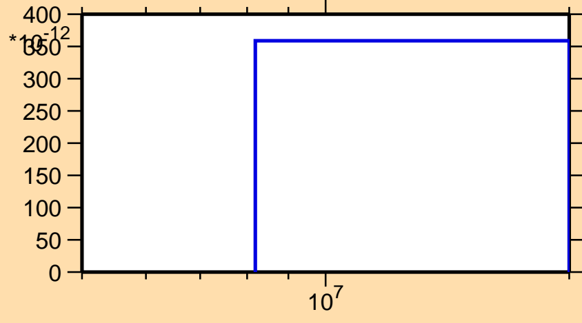
\sigma vs. E for ^{220}\text{Pb}(n,2n\alpha)
