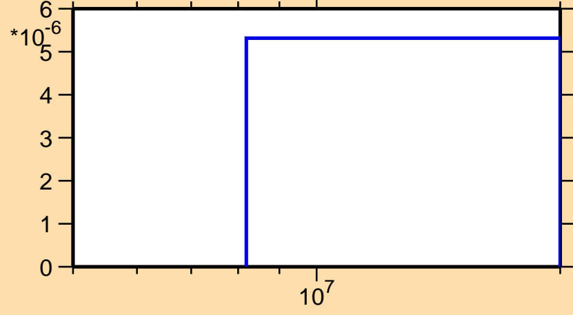
\sigma vs. E for ^{220}\text{Pb}(n,t)
