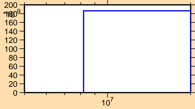
\sigma vs. E for ^{220}\text{Pb}(n,np)
