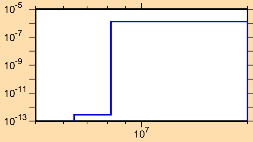
\sigma vs. E for ^{220}\text{Pb}(n,\alpha)
