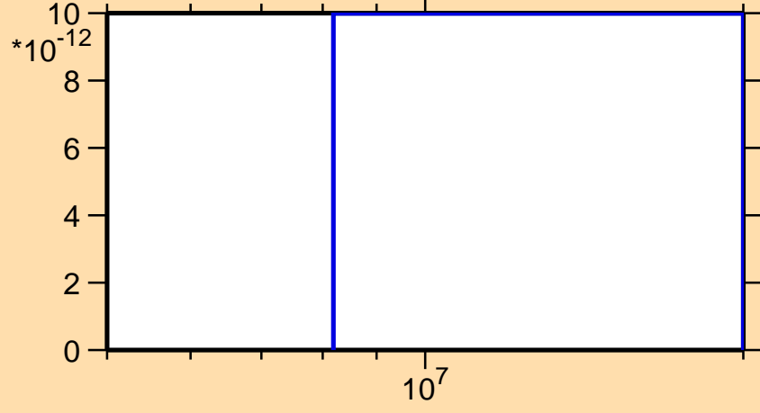
\sigma vs. E for ^{220}\text{Pb}(n,2np)
