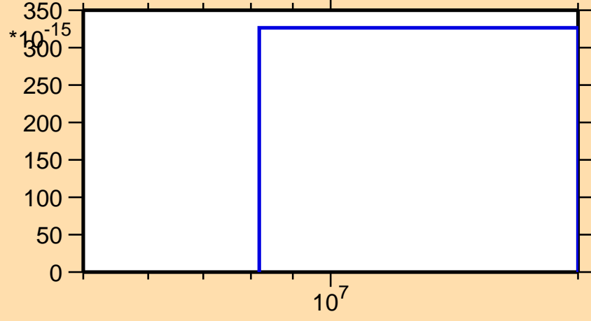
\sigma vs. E for ^{220}\text{Pb}(n,3n\alpha)
