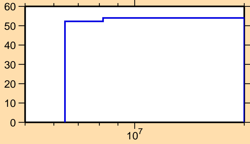
\Delta\sigma/\sigma vs. E for ^{220}\text{Pb}(n,\text{tot.})
