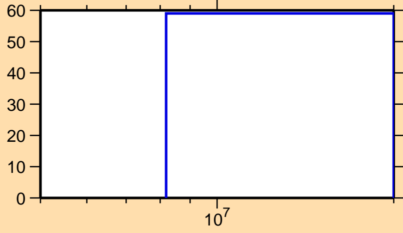
\Delta\sigma/\sigma vs. E for ^{220}\text{Pb}(n,\gamma)
