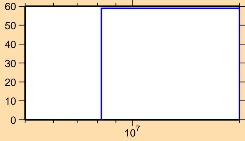
\Delta\sigma/\sigma vs. E for ^{220}\text{Pb}(n,\text{nonel.})
