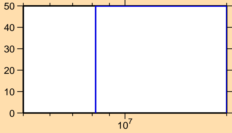
\Delta\sigma/\sigma vs. E for ^{220}\text{Pb}(n,el.)
