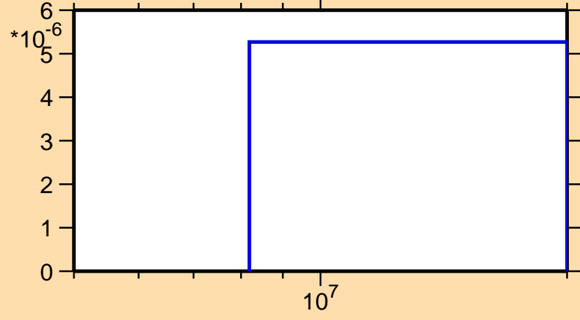
\sigma vs. E for ^{220}\text{Pb}(n,p)
