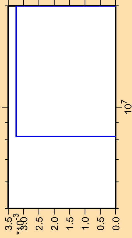
\Delta\sigma/\sigma vs. E for ^{220}\text{Pb} (mt 11)
