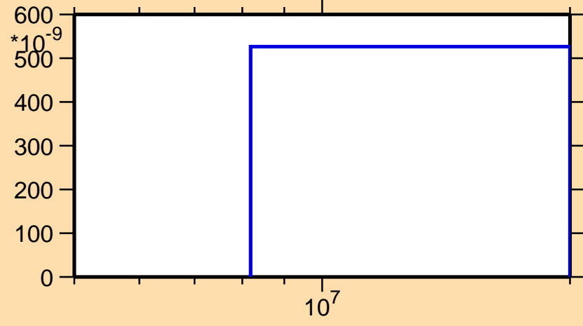
\sigma vs. E for ^{220}\text{Pb}(n,d)
