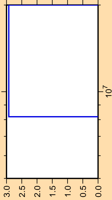
\Delta\sigma/\sigma vs. E for ^{220}\text{Pb}(n,3n\alpha)
