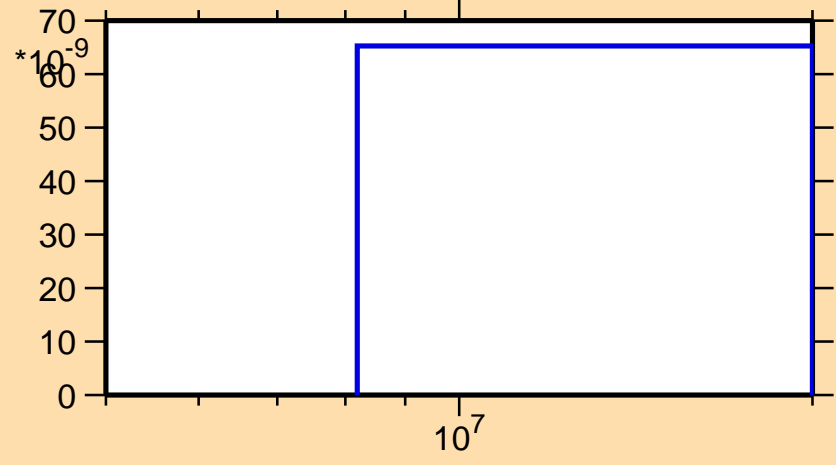
\sigma vs. E for ^{220}\text{Pb}(n,nt)
