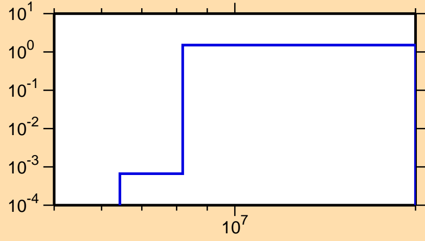
\sigma vs. E for ^{220}\text{Pb}(n,3n)
