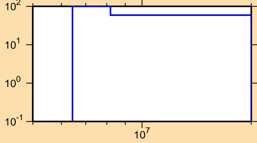
\Delta\sigma/\sigma vs. E for ^{220}\text{Pb}(n,\gamma)
