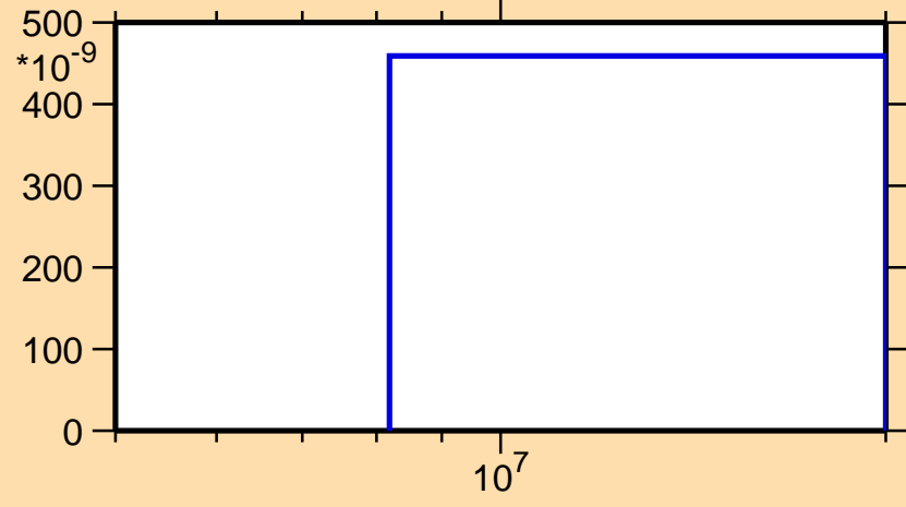
\sigma vs. E for ^{220}\text{Pb}(n,n\alpha)
