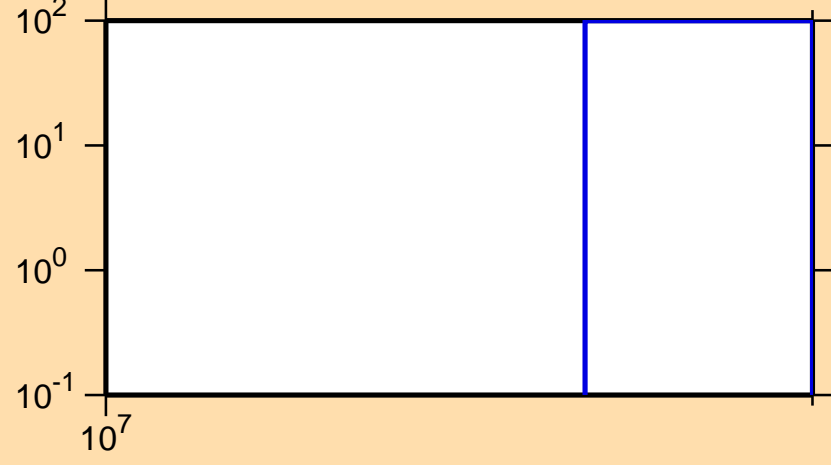
\Delta\sigma/\sigma vs. E for ^{92}\text{Pd}(n,2n)
