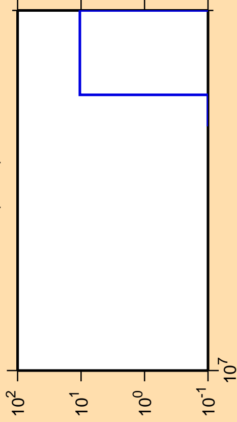
\Delta\sigma/\sigma vs. E for ^{92}\text{Pd}(n,\text{nd})
