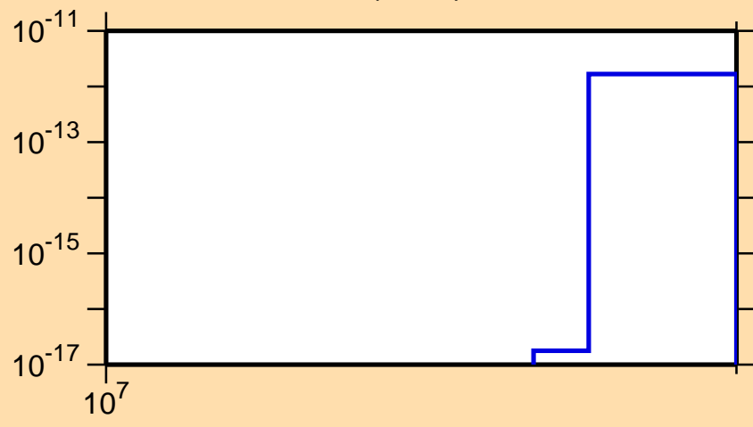
\sigma vs. E for ^{92}\text{Pd}(n,\text{nd})
