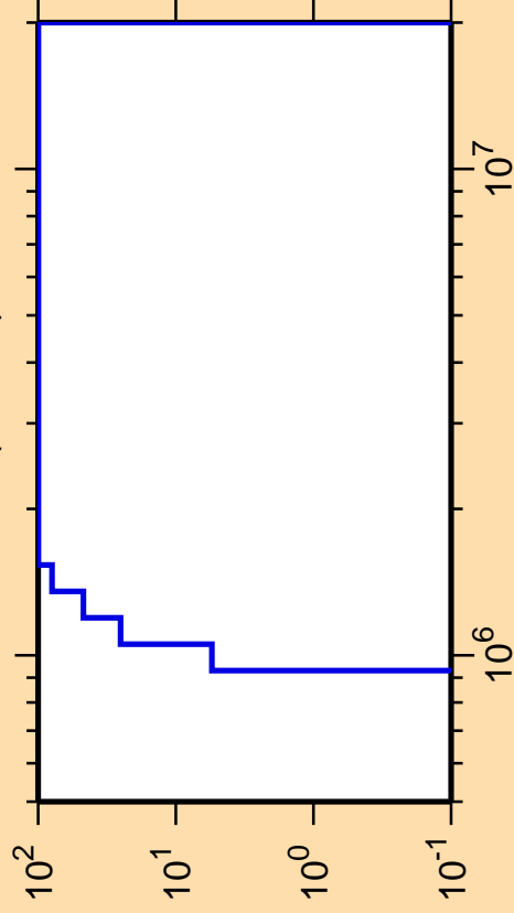
\Delta\sigma/\sigma vs. E for ^{92}\text{Pd}(n,\text{He3})
