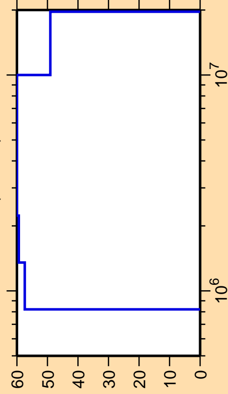
\Delta\sigma/\sigma vs. E for ^{92}\text{Pd}(n,\text{inel.})
