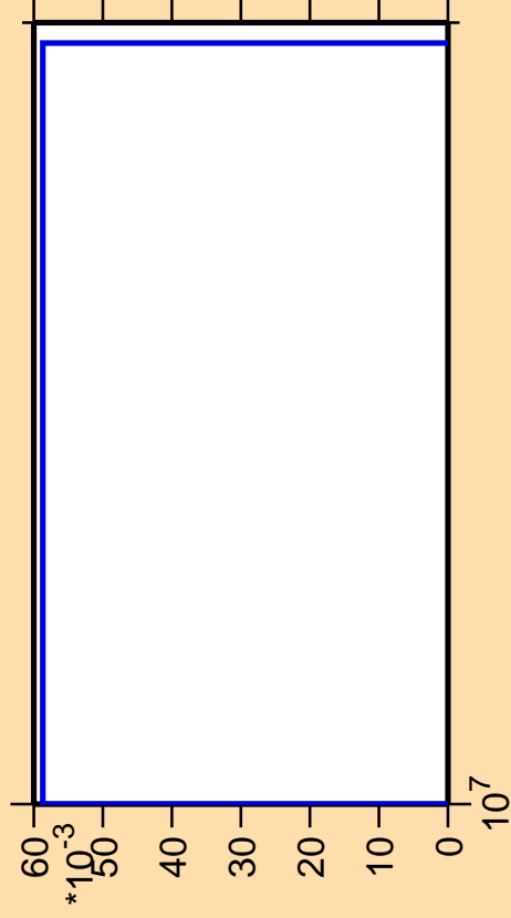
\Delta\sigma/\sigma vs. E for ^{92}\text{Pd}(n,\text{nd})
