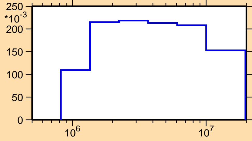
\sigma vs. E for ^{92}\text{Pd}(n,\text{inel.})
