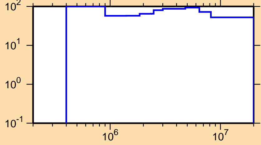
\Delta\sigma/\sigma vs. E for ^{92}\text{Pd}(n,\text{inel.})
