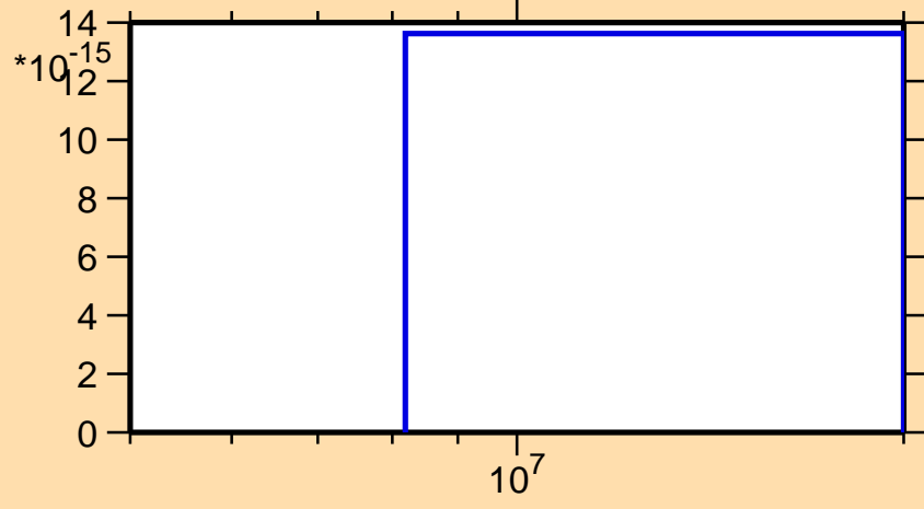
\sigma vs. E for ^{92}\text{Pd}(n,\text{nd})
