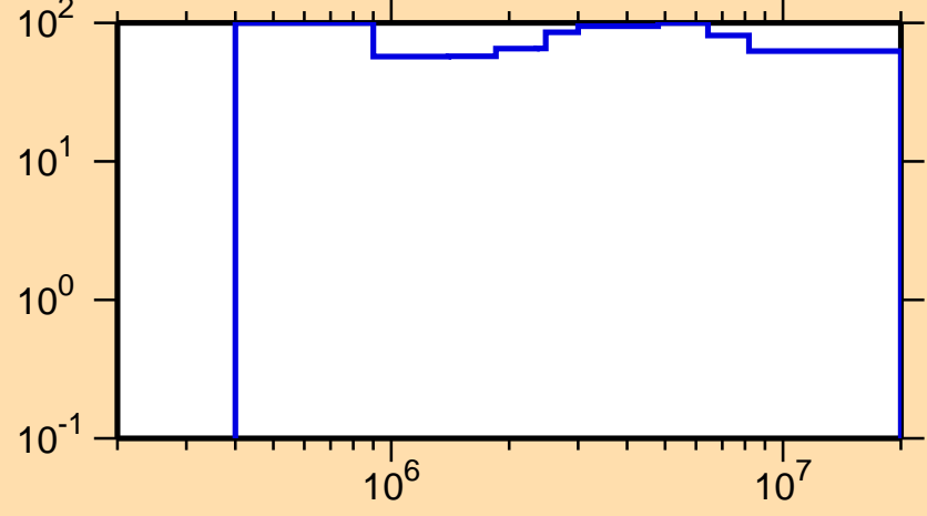
\Delta\sigma/\sigma vs. E for ^{92}\text{Pd}(n,n_1)
