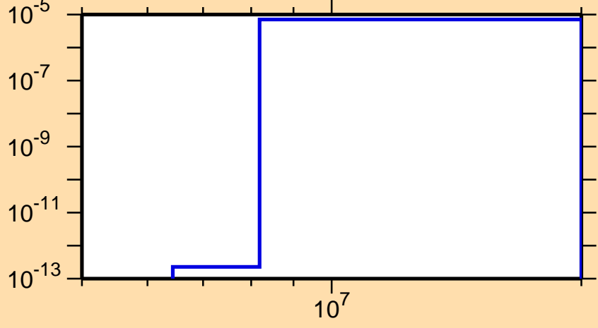
\sigma vs. E for ^{92}\text{Pd}(n,n\alpha)
