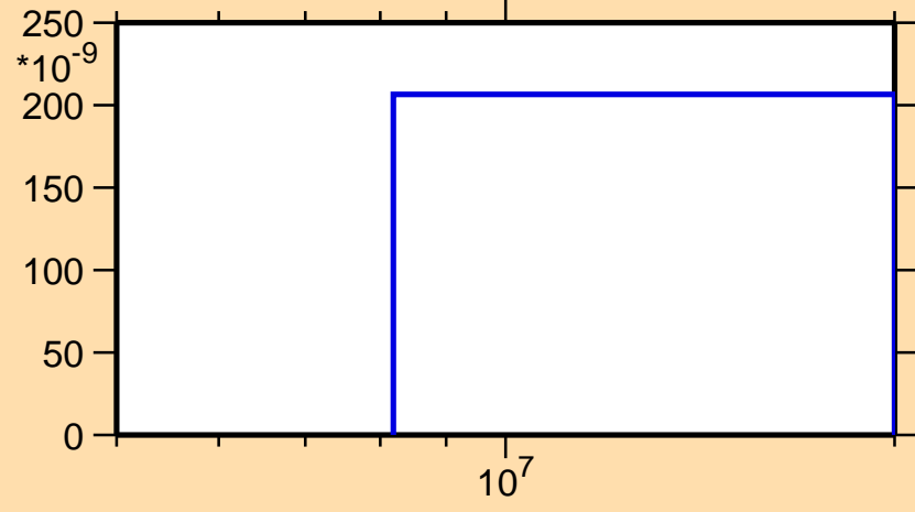
\sigma vs. E for ^{92}\text{Pd}(n,\text{pt})
