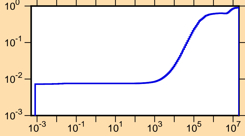
\mu vs. E for ^{93}\text{Pd}(\text{mt251})
