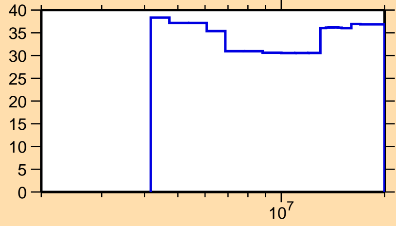
\Delta\sigma/\sigma vs. E for ^{93}\text{Pd}(n,n\text{nonel.})
