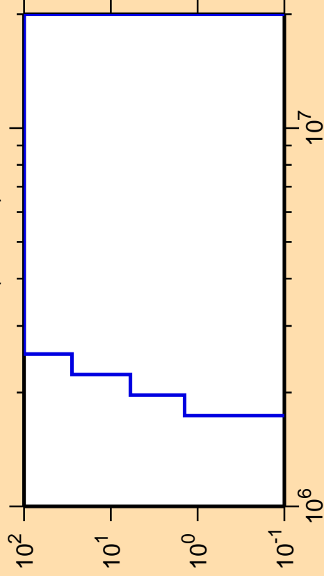
\Delta\sigma/\sigma vs. E for ^{93}\text{Pd}(n,\text{He3})
