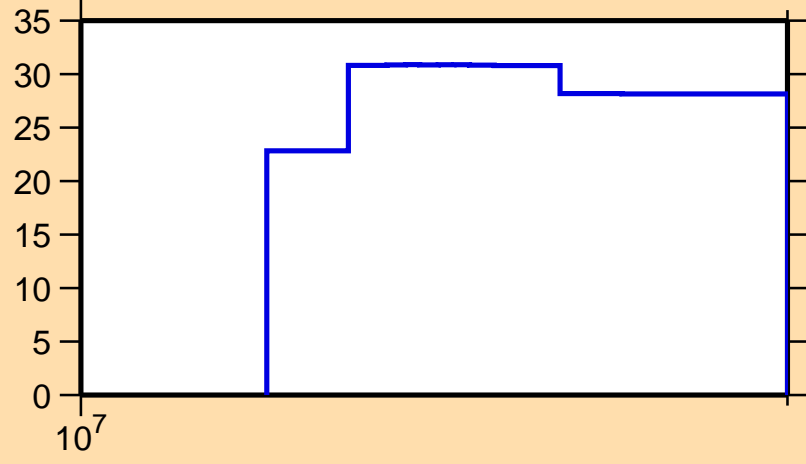
\Delta\sigma/\sigma vs. E for ^{93}\text{Pd}(n,\text{tot.})
