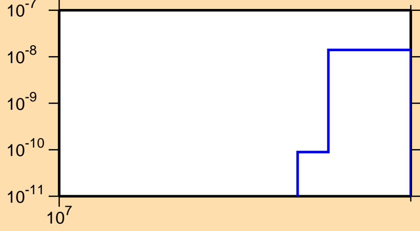
\sigma vs. E for ^{93}\text{Pd}(n,\text{nd})
