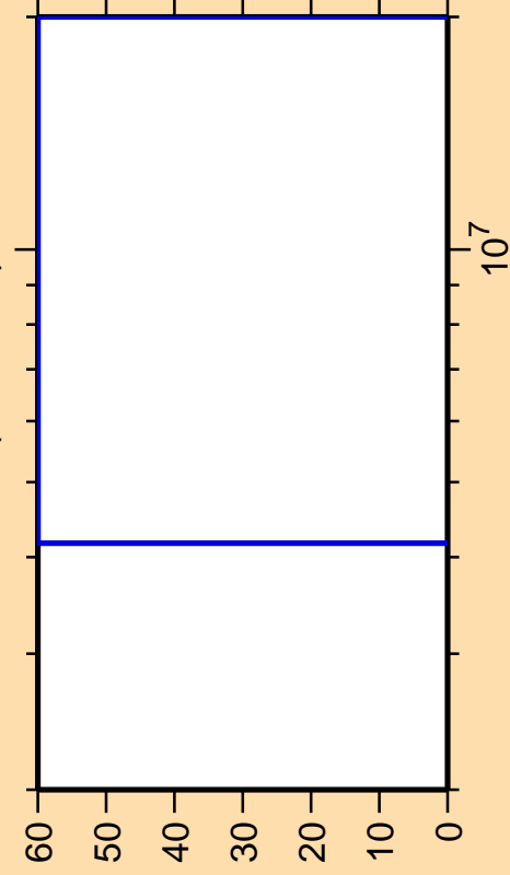
\Delta\sigma/\sigma vs. E for ^{93}\text{Pd}(n,\text{ncont.})
