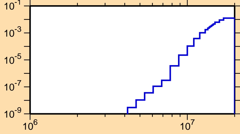
\sigma vs. E for ^{93}\text{Pd}(n,\text{He3})
