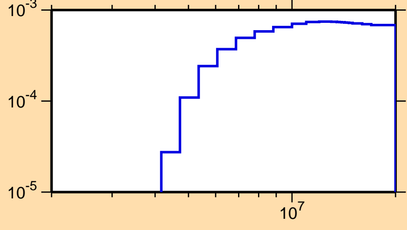
\sigma vs. E for ^{93}\text{Pd}(n,n\text{cont.})
