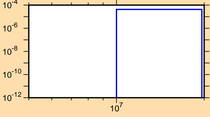
\sigma vs. E for ^{93}\text{Pd}(n,t)
