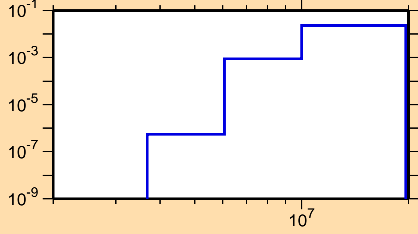
\sigma vs. E for ^{93}\text{Pd}(n,d)
