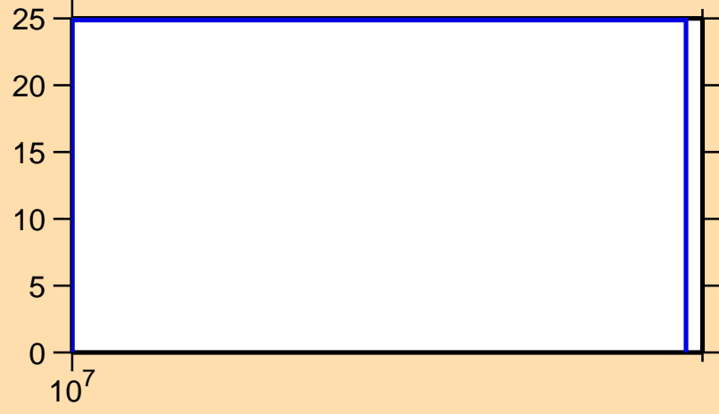
\Delta\sigma/\sigma vs. E for ^{93}\text{Pd}(n,\text{el.})
