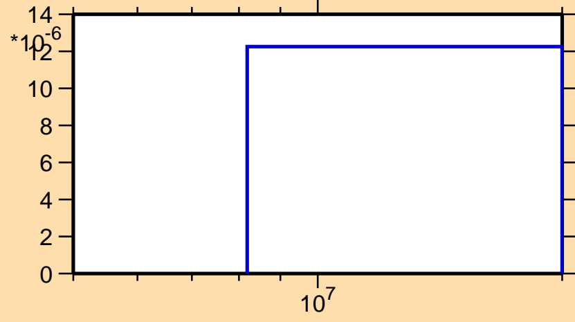
\sigma vs. E for ^{93}\text{Pd}(n,2n)
