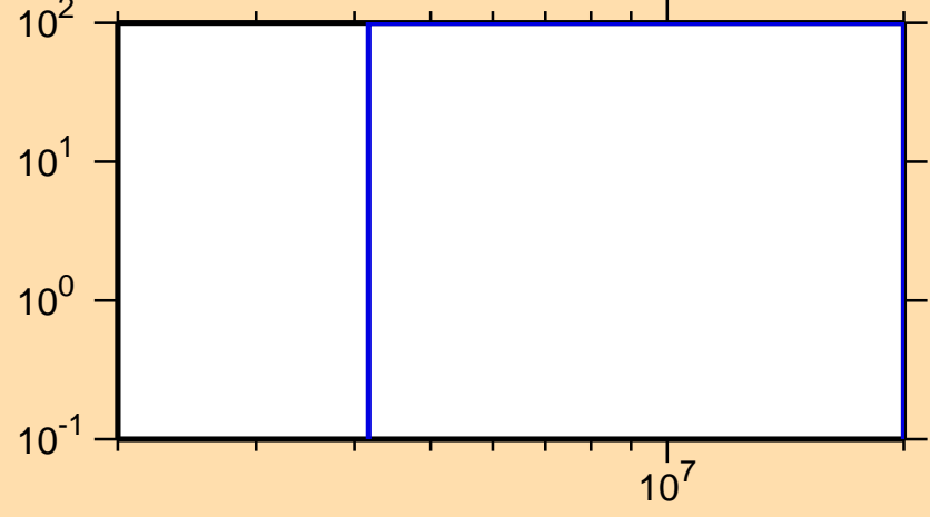
\Delta\sigma/\sigma vs. E for ^{94}\text{Pd}(n,n\text{cont.})
