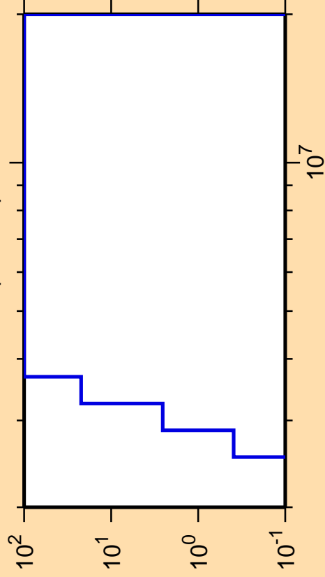
\Delta\sigma/\sigma vs. E for ^{94}\text{Pd}(n,\text{He3})
