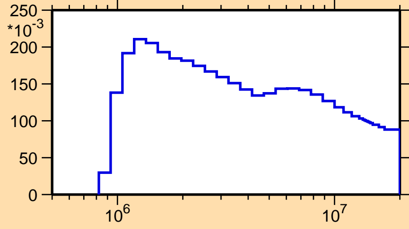
\sigma vs. E for ^{94}\text{Pd}(n,\text{inel.})
