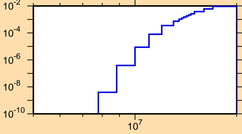
\sigma vs. E for ^{94}\text{Pd}(n,pd)
