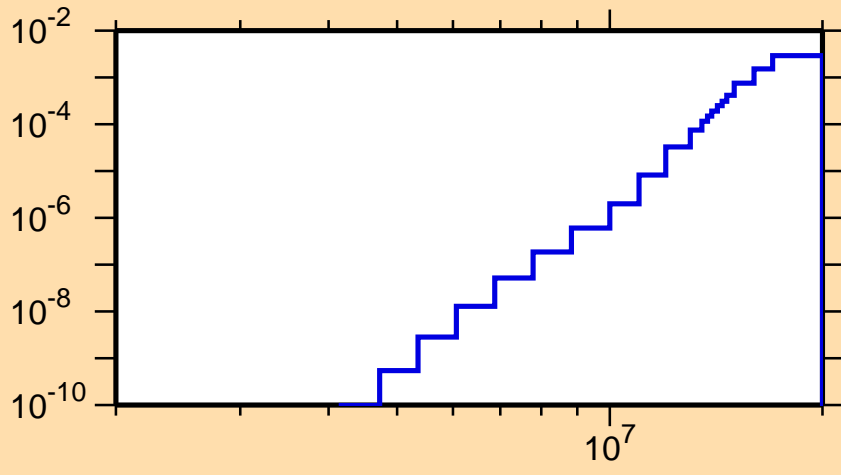
\sigma vs. E for ^{94}\text{Pd}(n,\text{He3})
