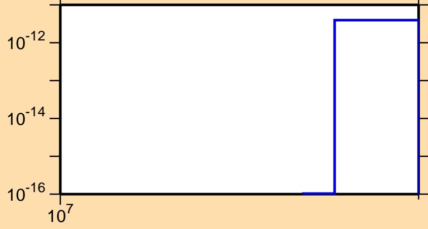
\sigma vs. E for ^{94}\text{Pd}(\text{mt } 34)
