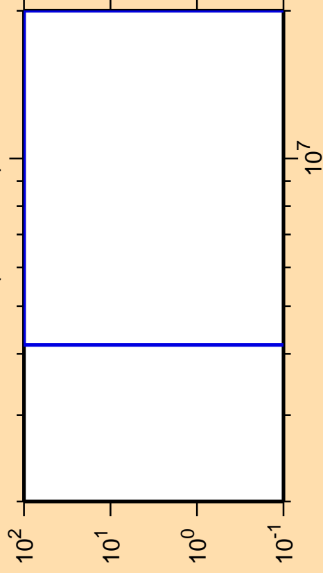
\Delta\sigma/\sigma vs. E for ^{94}\text{Pd}(n,\text{ncont.})
