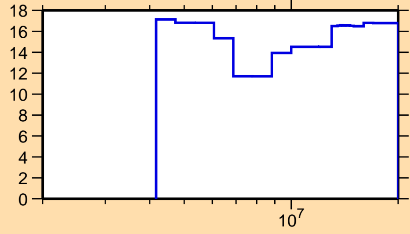
\Delta\sigma/\sigma vs. E for ^{94}\text{Pd}(n,n\text{nonel.})
