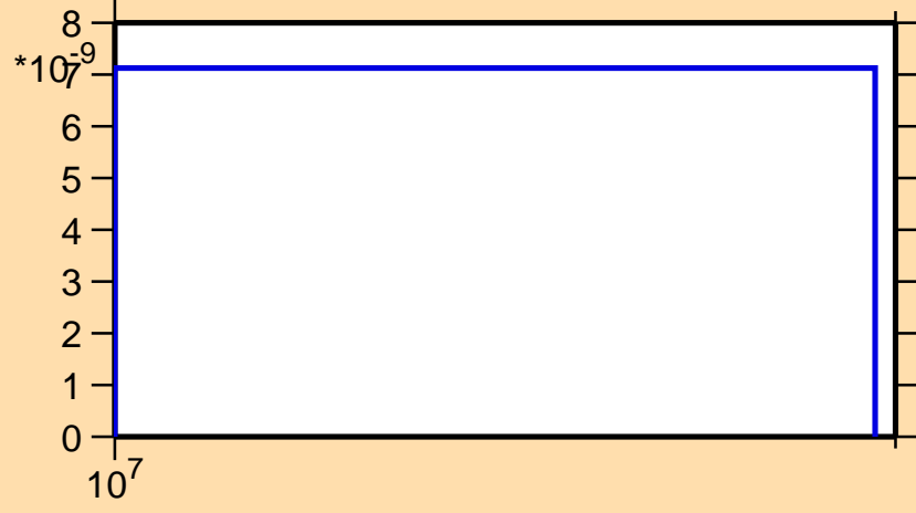
\sigma vs. E for ^{94}\text{Pd}(n,\text{pt})
