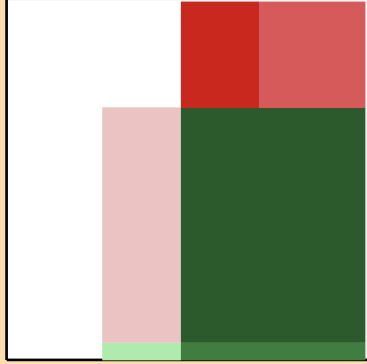
\Delta\sigma/\sigma vs. E for ^{94}\text{Pd}(n,ncont.)
