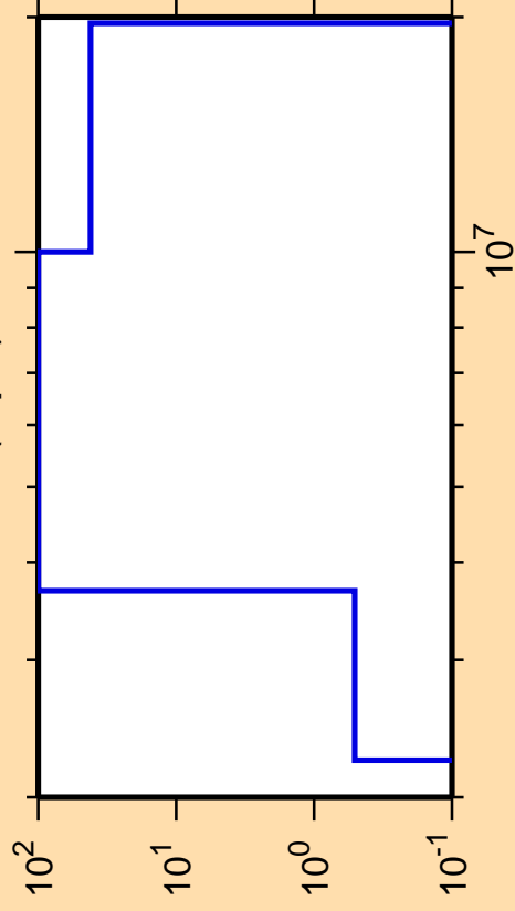
\Delta\sigma/\sigma vs. E for ^{94}\text{Pd}(n,p\alpha)
