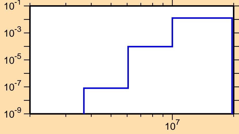
\sigma vs. E for ^{94}\text{Pd}(n,d)
