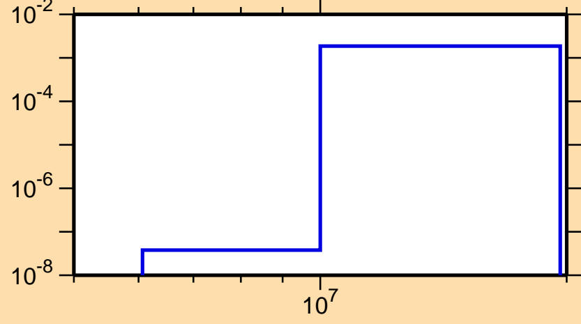
\sigma vs. E for ^{94}\text{Pd}(n,\text{pd})
