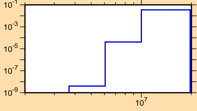
\sigma vs. E for ^{94}\text{Pd}(n,p\alpha)
