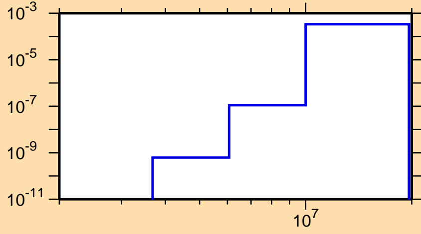
\sigma vs. E for ^{94}\text{Pd}(n,\text{He3})
