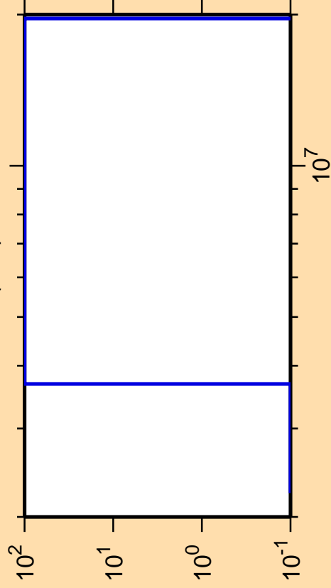
\Delta\sigma/\sigma vs. E for ^{95}\text{Pd}(n,d)
