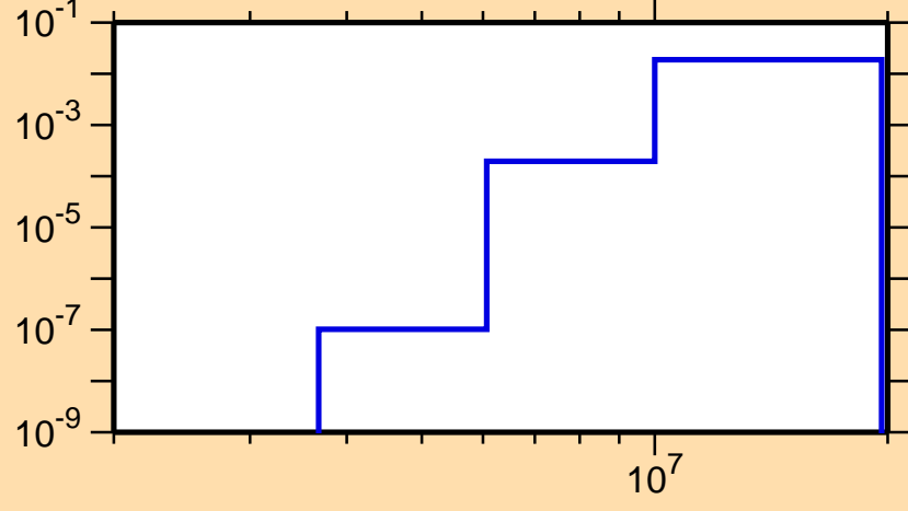
\sigma vs. E for ^{95}\text{Pd}(n,d)
