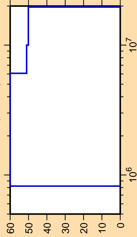
\Delta\sigma/\sigma vs. E for ^{95}\text{Pd}(n,\text{inel.})
