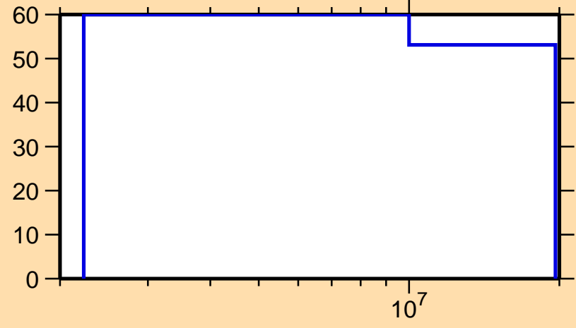
\Delta\sigma/\sigma vs. E for ^{95}\text{Pd}(n,n\text{cont.})
