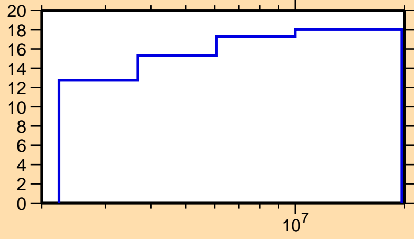
\Delta\sigma/\sigma vs. E for ^{95}\text{Pd}(n,n\text{nonel.})
