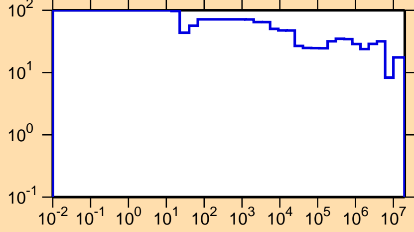
\Delta\sigma/\sigma vs. E for ^{95}\text{Pd}(n,\text{el.})
