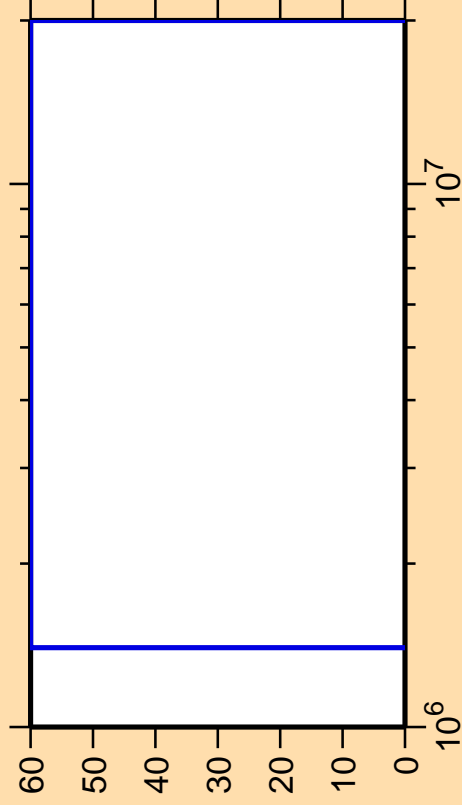
\Delta\sigma/\sigma vs. E for ^{95}\text{Pd}(n,n_3)
