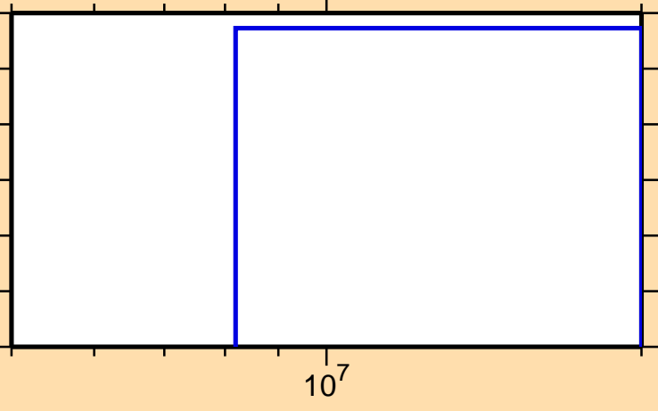
\sigma vs. E for ^{95}\text{Pd}(n,2n)
