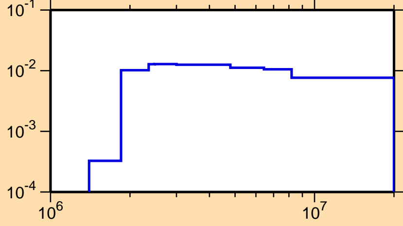
\sigma vs. E for ^{95}\text{Pd}(n,n_3)
