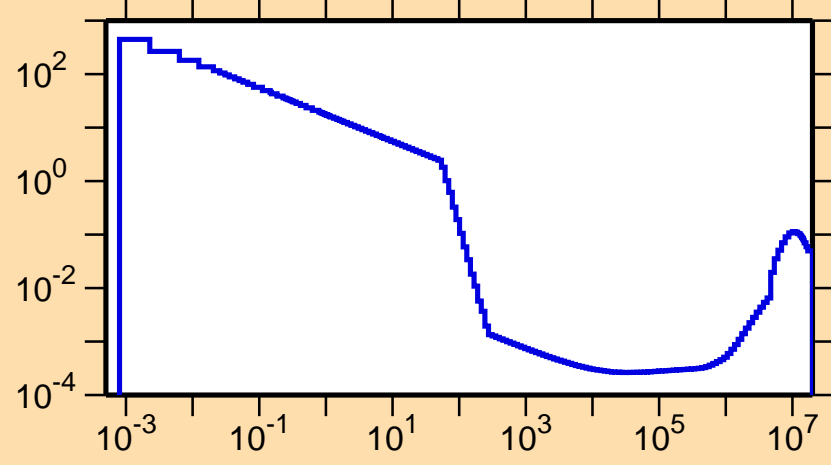
\sigma vs. E for ^{95}\text{Pd}(n,\alpha)
