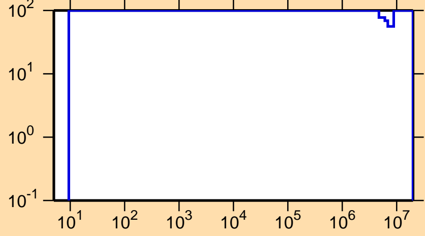
\Delta\sigma/\sigma vs. E for ^{95}\text{Pd}(n,\gamma)
