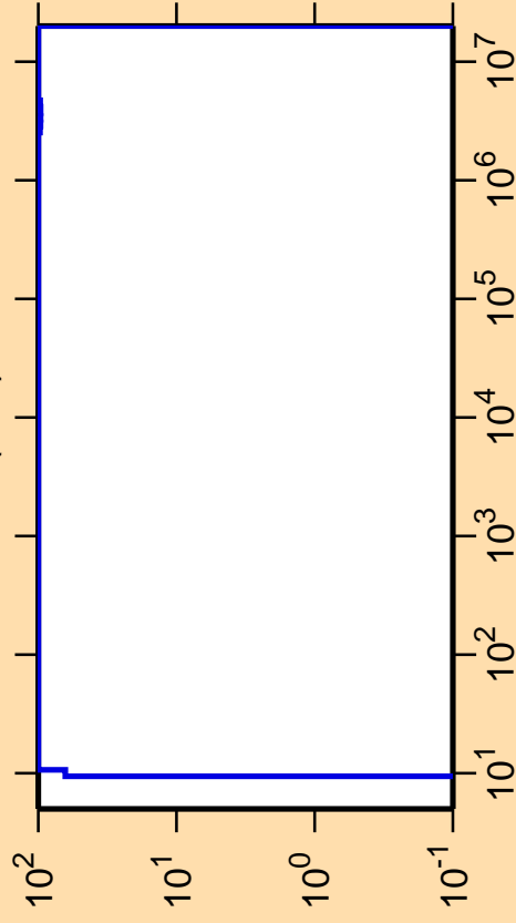
\Delta\sigma/\sigma vs. E for ^{95}\text{Pd}(n,\alpha)
