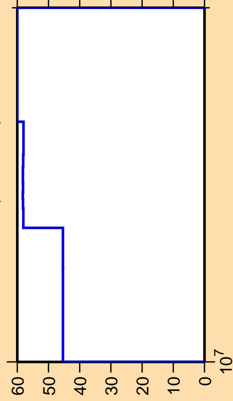
\Delta\sigma/\sigma vs. E for ^{95}\text{Pd}(n,ncont.)
