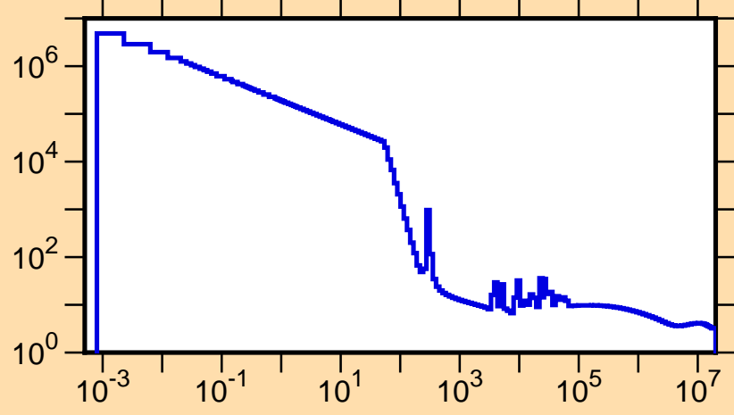
\sigma vs. E for ^{95}\text{Pd}(n,\text{tot.})
