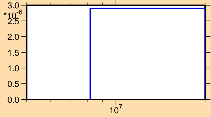
\sigma vs. E for ^{95}\text{Pd}(n,\text{pt})
