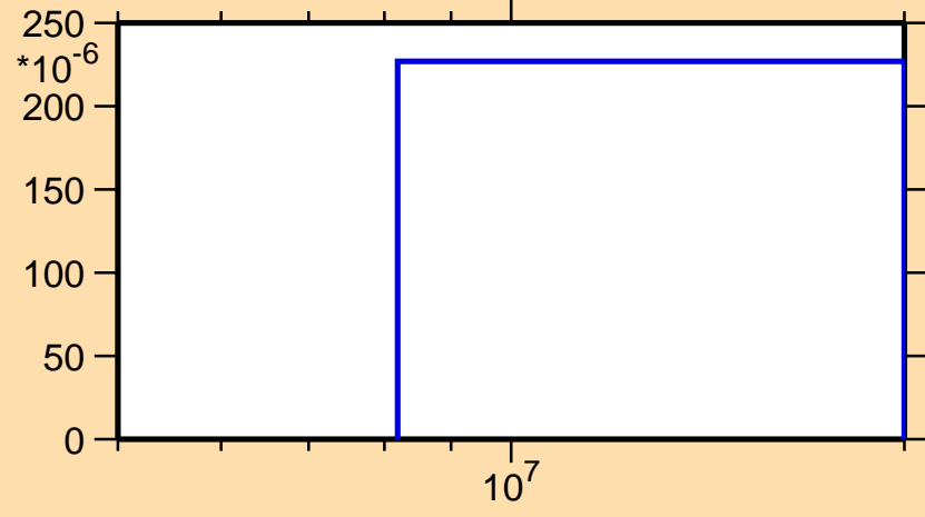
\sigma vs. E for ^{95}\text{Pd}(n,2n)
