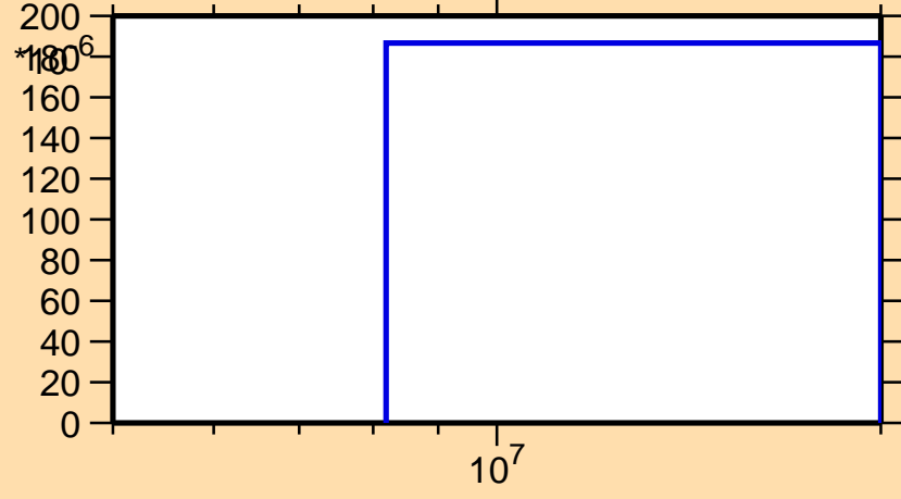
\sigma vs. E for ^{95}\text{Pd}(n,t)
