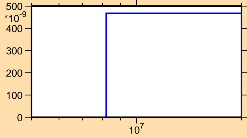
\sigma vs. E for ^{95}\text{Pd}(n,2np)
