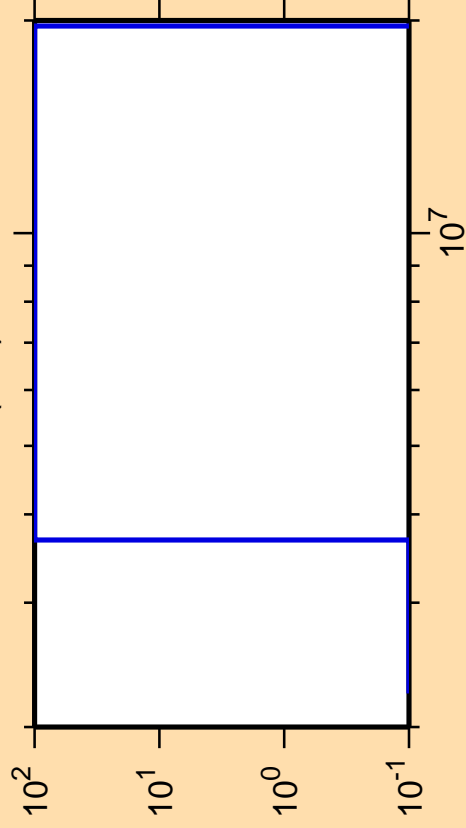
\Delta\sigma/\sigma vs. E for ^{96}\text{Pd}(n,d)
