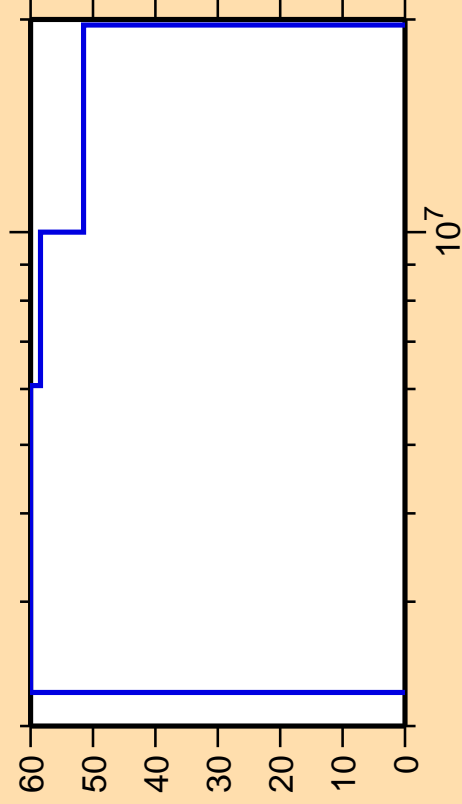
\Delta\sigma/\sigma vs. E for ^{96}\text{Pd}(n,n_3)
