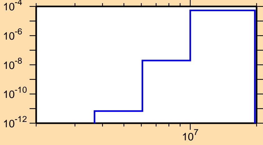
\sigma vs. E for ^{96}\text{Pd}(n,\text{He3})
