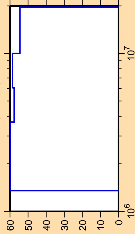
\Delta\sigma/\sigma vs. E for ^{96}\text{Pd}(n,\text{inel.})
