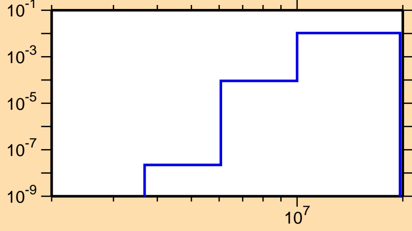
\sigma vs. E for ^{96}\text{Pd}(n,d)
