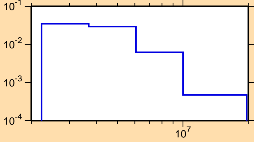
\sigma vs. E for ^{96}\text{Pd}(n,n_3)
