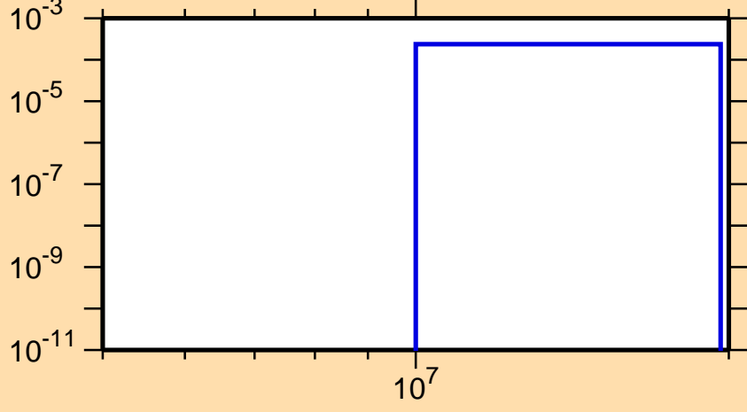
\sigma vs. E for ^{96}\text{Pd}(n,\text{pd})
