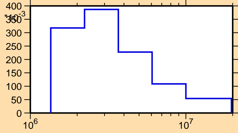
\sigma vs. E for ^{96}\text{Pd}(n,\text{inel.})
