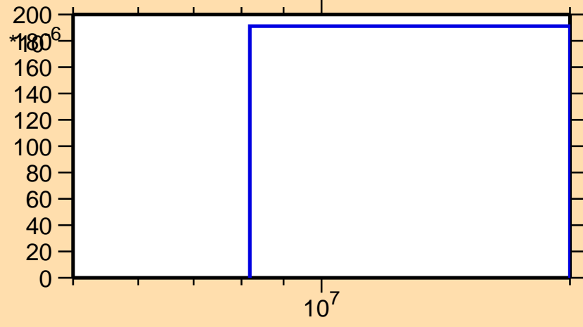
\sigma vs. E for ^{96}\text{Pd}(n,\text{pd})
