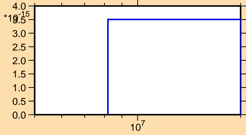
\sigma vs. E for ^{96}\text{Pd}(n,2np)
