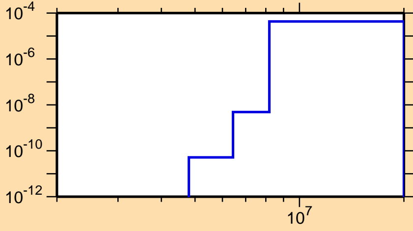
\sigma vs. E for ^{96}\text{Pd}(n,\text{He3})
