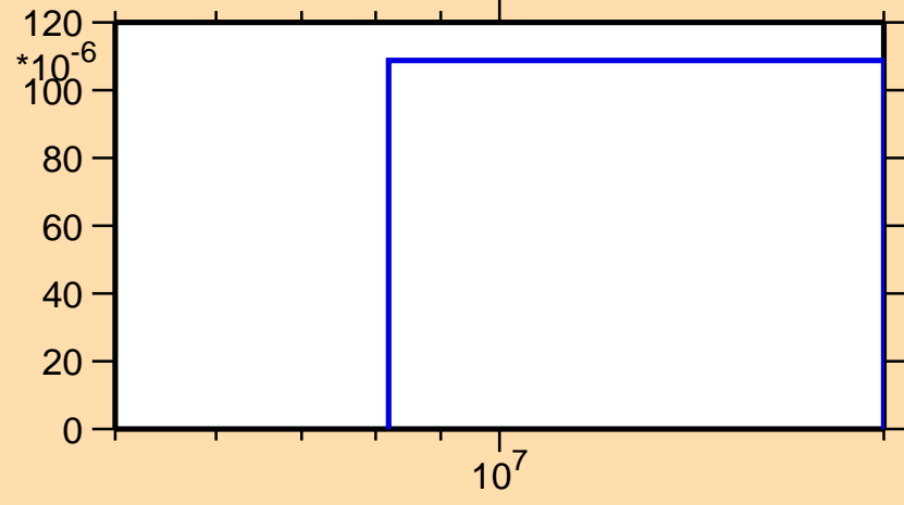
\sigma vs. E for ^{96}\text{Pd}(n,2n)
