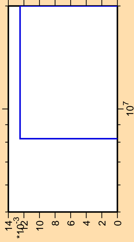
\Delta\sigma/\sigma vs. E for ^{96}\text{Pd}(\text{mt } 34)
