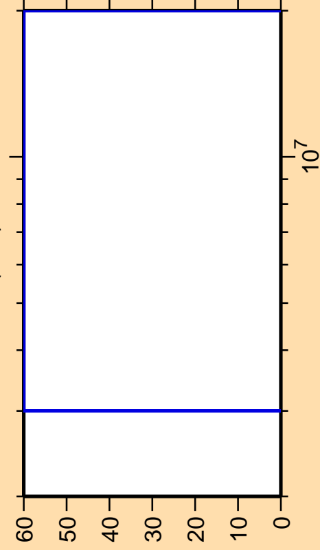
\Delta\sigma/\sigma vs. E for ^{96}\text{Pd}(n,\alpha)
