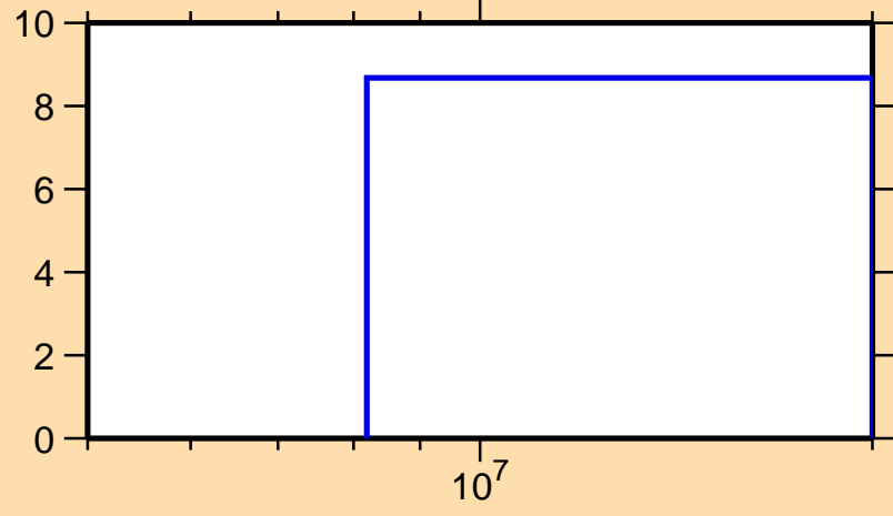
\Delta\sigma/\sigma vs. E for ^{96}\text{Pd}(n,\text{tot.})
