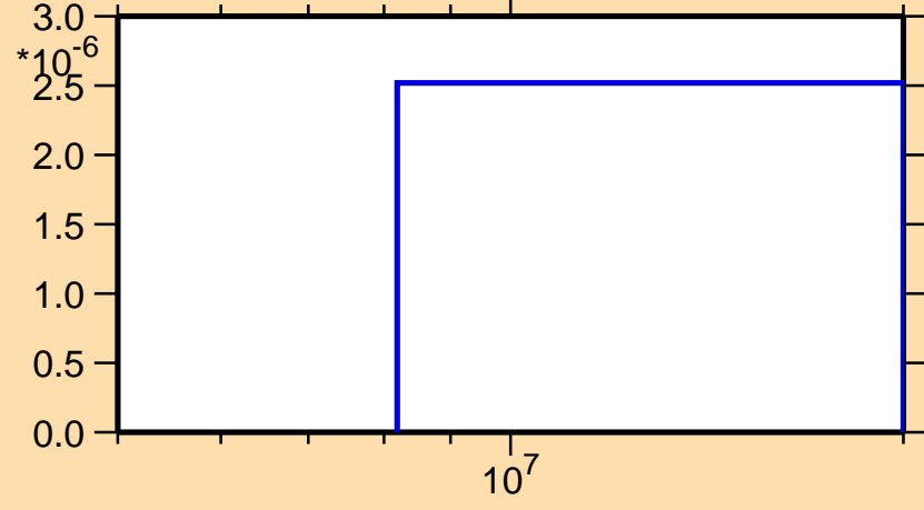
\sigma vs. E for ^{96}\text{Pd}(n,t)
