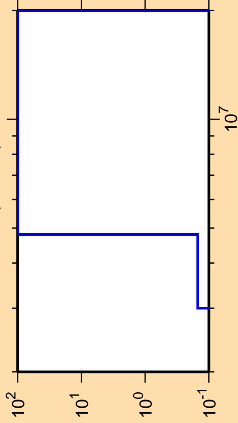
\Delta\sigma/\sigma vs. E for ^{96}\text{Pd}(n,\text{He3})
