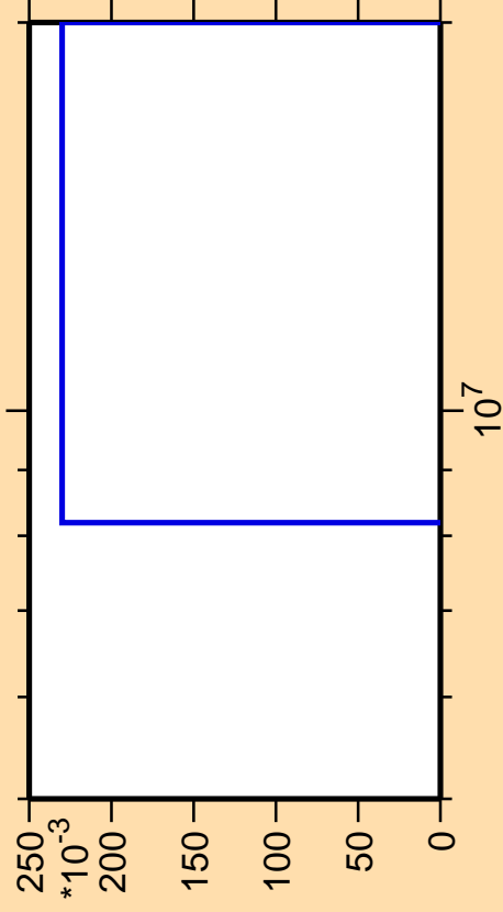
\Delta\sigma/\sigma vs. E for ^{96}\text{Pd}(\text{mt117})
