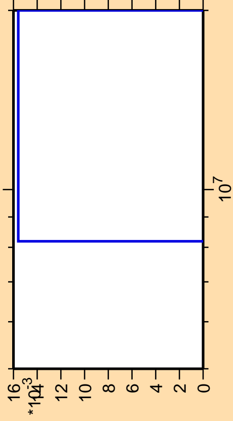
\Delta\sigma/\sigma vs. E for ^{96}\text{Pd}(n,2np)
