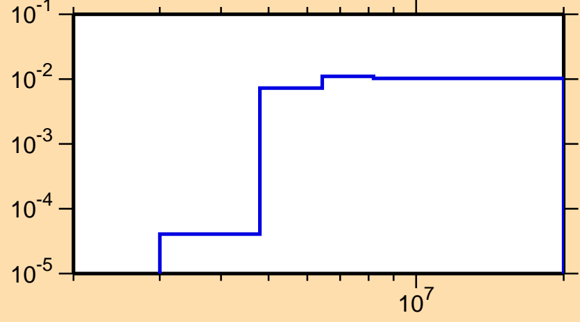
\sigma vs. E for ^{96}\text{Pd}(n,n\text{cont.})
