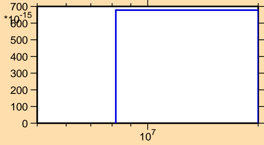
\sigma vs. E for ^{96}\text{Pd}(n,\text{nd})
