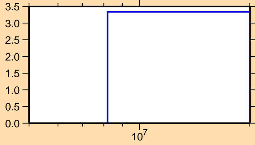
\Delta\sigma/\sigma vs. E for ^{96}\text{Pd}(n,\text{nonel.})
