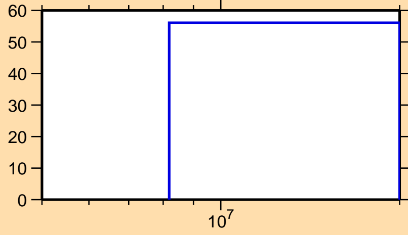
\Delta\sigma/\sigma vs. E for ^{96}\text{Pd}(n,\text{inel.})
