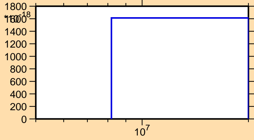
\sigma vs. E for ^{96}\text{Pd}(\text{mt } 34)
