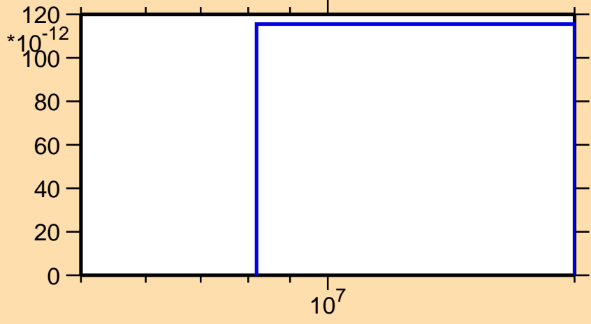
\sigma vs. E for ^{96}\text{Pd}(n,\text{pt})
