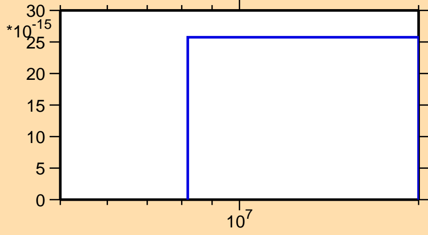
\sigma vs. E for ^{96}\text{Pd}(\text{mt117})
