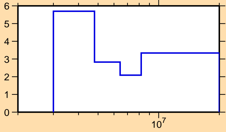
\Delta\sigma/\sigma vs. E for ^{96}\text{Pd}(n,n\text{nonel.})
