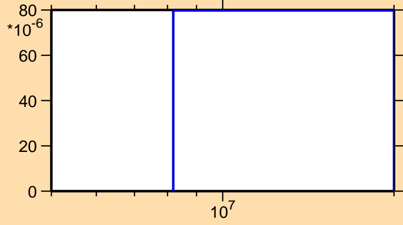
\sigma vs. E for ^{96}\text{Pd}(n,n\alpha)
