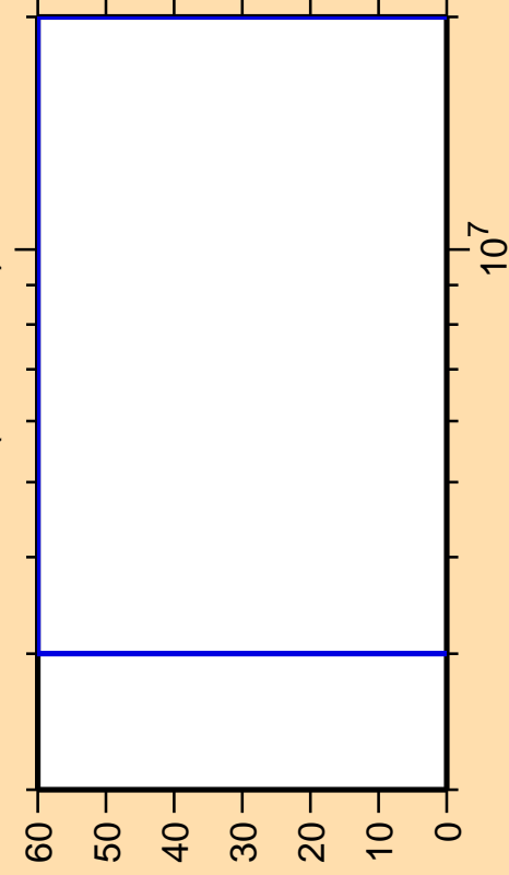
\Delta\sigma/\sigma vs. E for ^{96}\text{Pd}(n,n\text{cont.})
