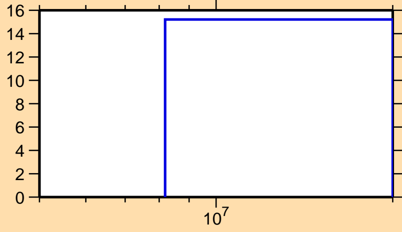
\Delta\sigma/\sigma vs. E for ^{96}\text{Pd}(n,\text{el.})
