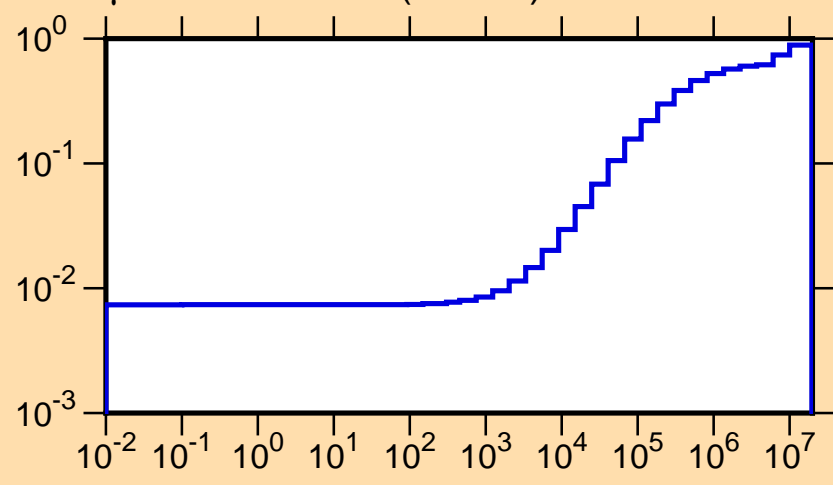
\mu vs. E for ^{97}\text{Pd}(\text{mt251})
