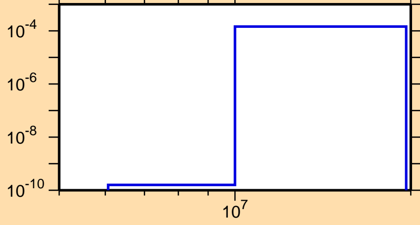
\sigma vs. E for ^{97}\text{Pd}(n,t)
