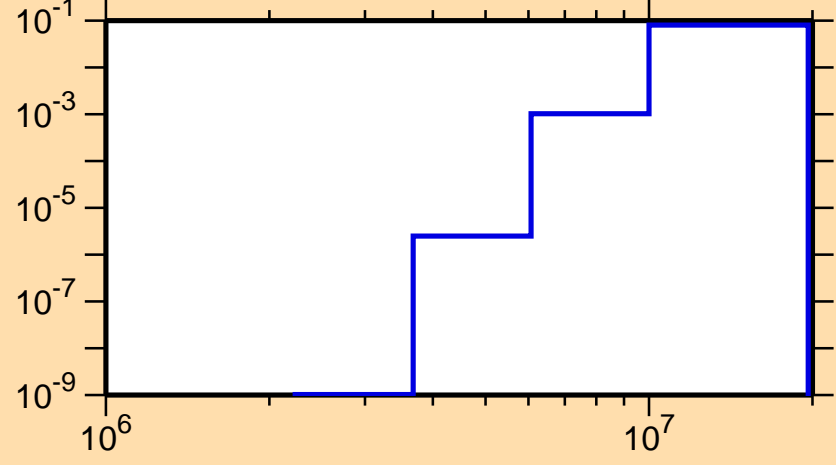
\sigma vs. E for ^{97}\text{Pd}(n,p\alpha)
