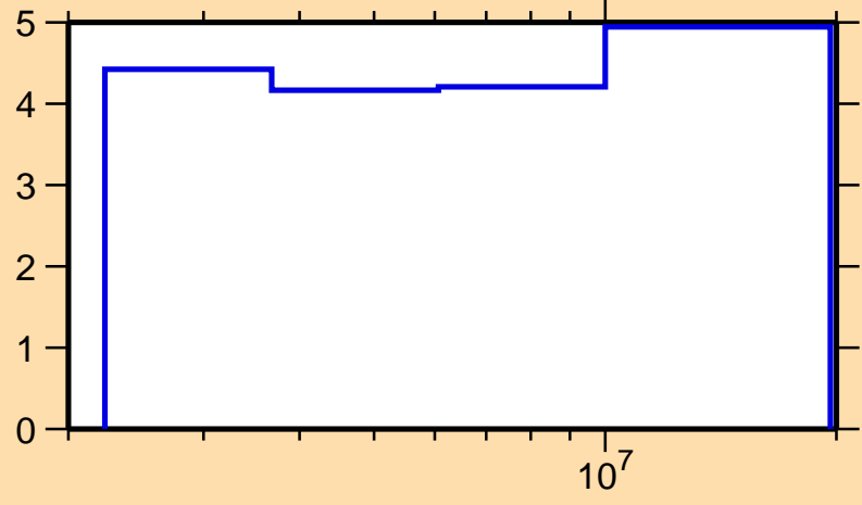
\Delta\sigma/\sigma vs. E for ^{97}\text{Pd}(n,n\text{nonel.})
