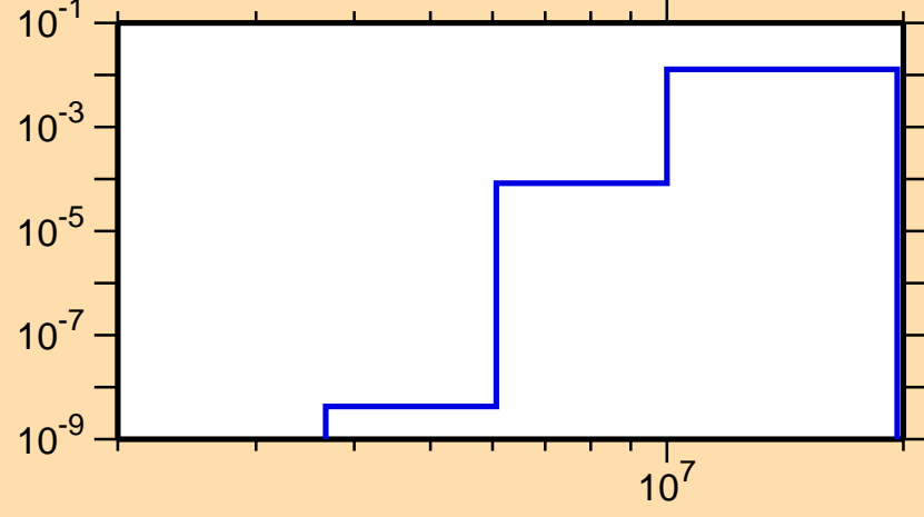
\sigma vs. E for ^{97}\text{Pd}(n,d)
