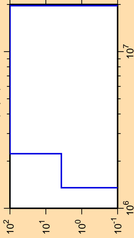
\Delta\sigma/\sigma vs. E for ^{97}\text{Pd}(n,p\alpha)
