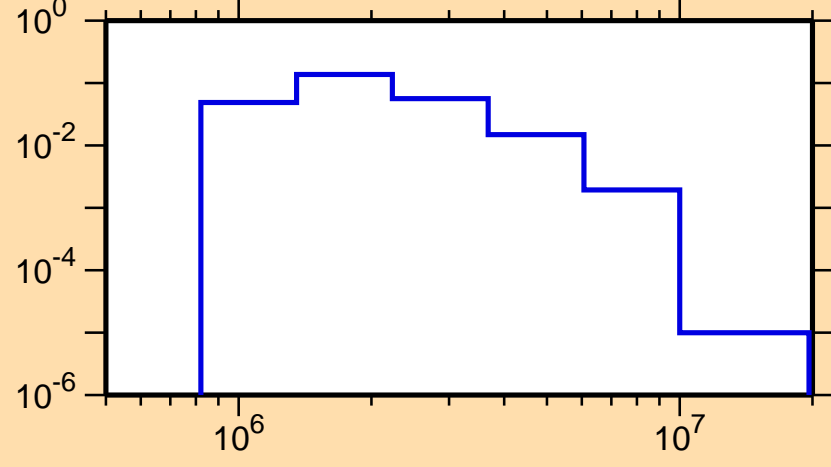
\sigma vs. E for ^{97}\text{Pd}(n,n_3)
