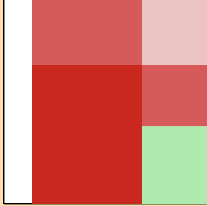
\Delta\sigma/\sigma vs. E for ^{98}\text{Pd}(n,2n)
