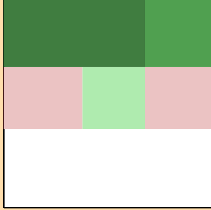
\Delta\sigma/\sigma vs. E for ^{98}\text{Pd}(n,\text{tot.})
