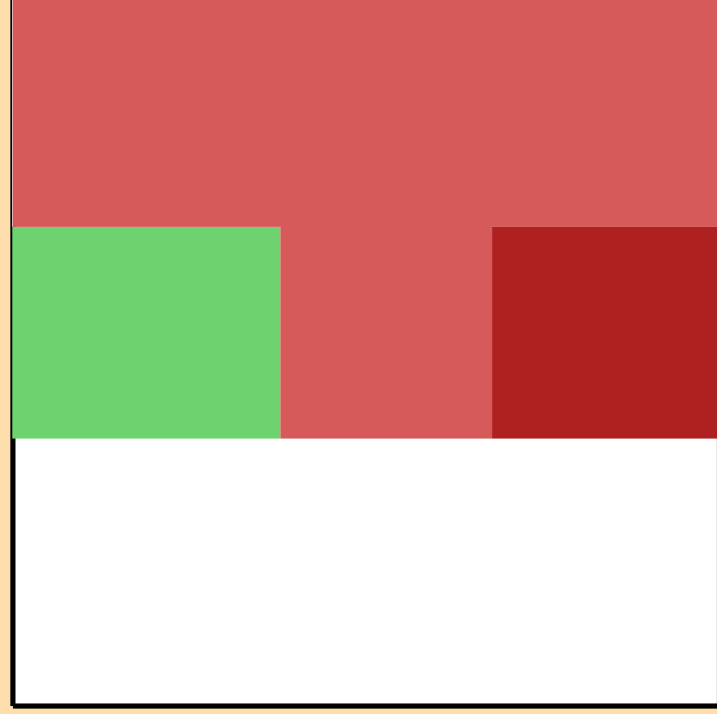
\Delta\sigma/\sigma vs. E for ^{98}\text{Pd}(n,\text{inel.})
