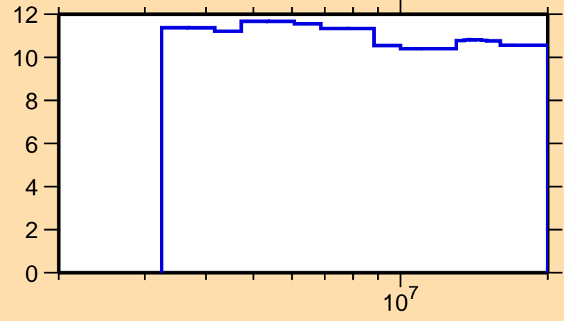
\Delta\sigma/\sigma vs. E for ^{98}\text{Pd}(n,n\text{nonel.})
