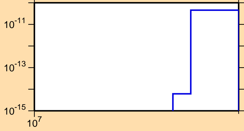
\sigma vs. E for ^{98}\text{Pd}(\text{mt } 34)
