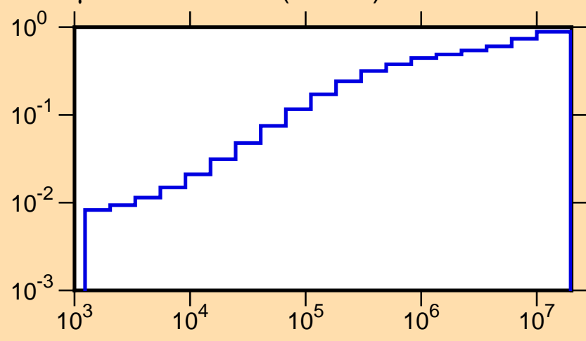
\mu vs. E for ^{98}\text{Pd}(\text{mt251})
