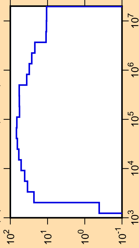
\Delta\mu/\mu vs. E for ^{98}\text{Pd}(\text{mt251})
