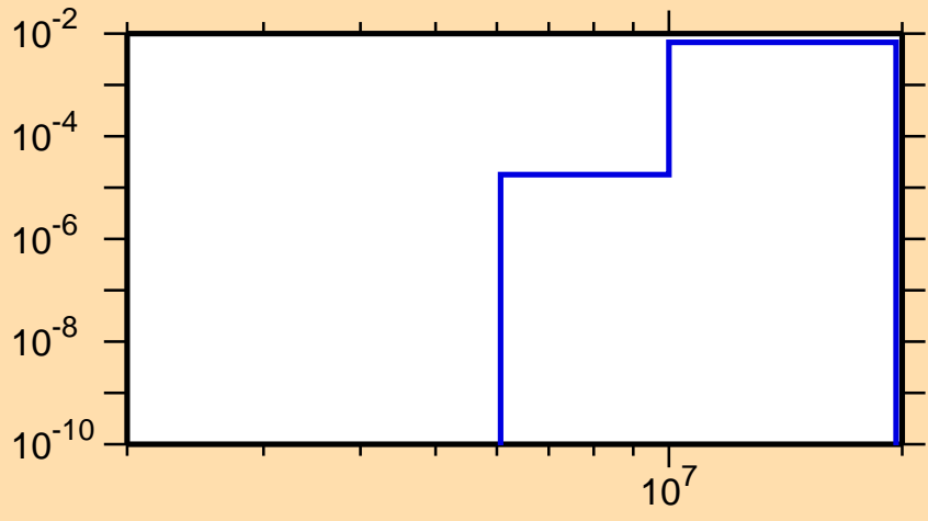
\sigma vs. E for ^{98}\text{Pd}(n,d)
