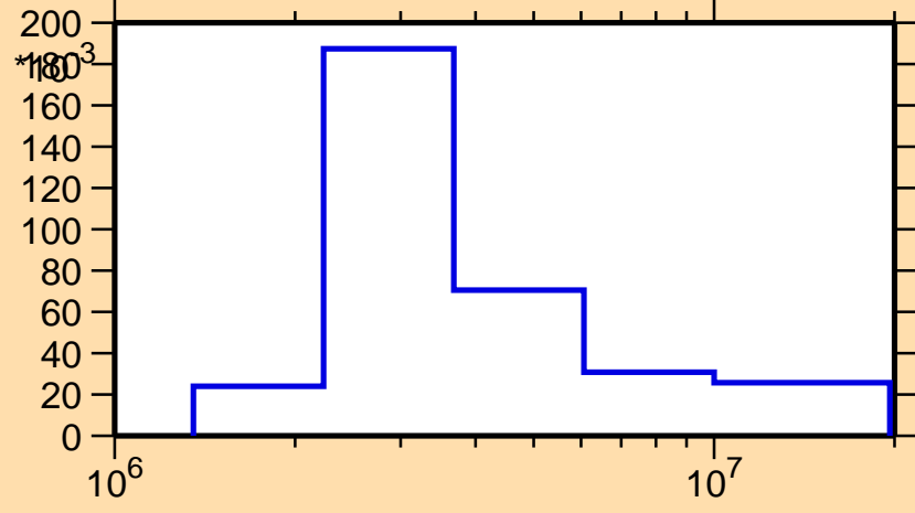
\sigma vs. E for ^{98}\text{Pd}(n,n_3)
