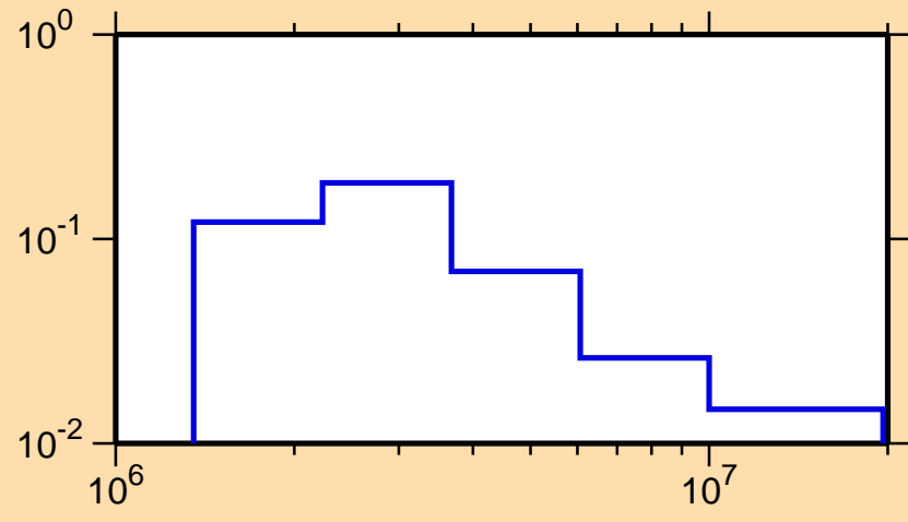
\sigma vs. E for ^{98}\text{Pd}(n,n_2)
