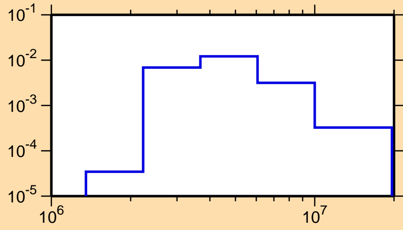
\sigma vs. E for ^{98}\text{Pd}(n,n_4)
