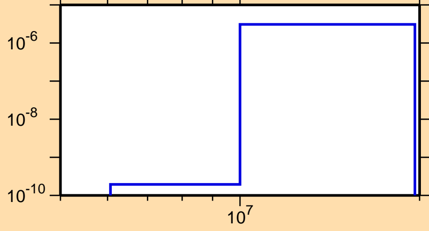
\sigma vs. E for ^{98}\text{Pd}(n,\text{He3})
