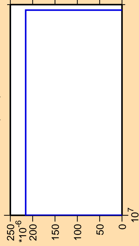
\Delta\sigma/\sigma vs. E for ^{98}\text{Pd}(n,nt)
