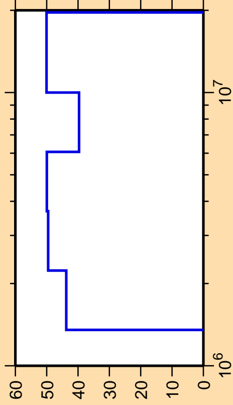
\Delta\sigma/\sigma vs. E for ^{98}\text{Pd}(n,n_4)
