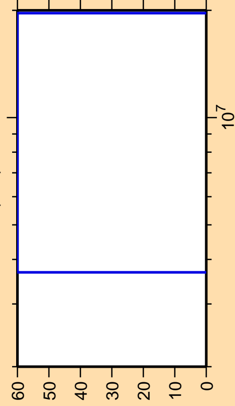
\Delta\sigma/\sigma vs. E for ^{98}\text{Pd}(n,d)
