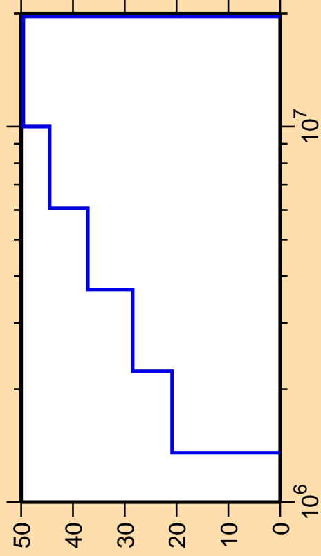
\Delta\sigma/\sigma vs. E for ^{98}\text{Pd}(n,n_2)
