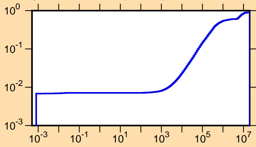
\mu vs. E for ^{99}\text{Pd}(\text{mt251})
