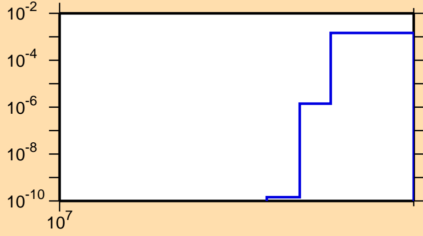
\sigma vs. E for ^{99}\text{Pd}(n,2np)
