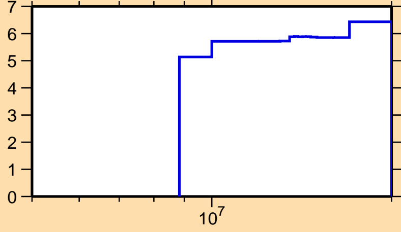
\Delta\sigma/\sigma vs. E for ^{99}\text{Pd}(n,\text{nonel.})
