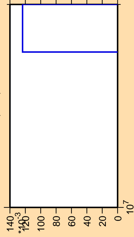
\Delta\sigma/\sigma vs. E for ^{99}\text{Pd}(n,nt)
