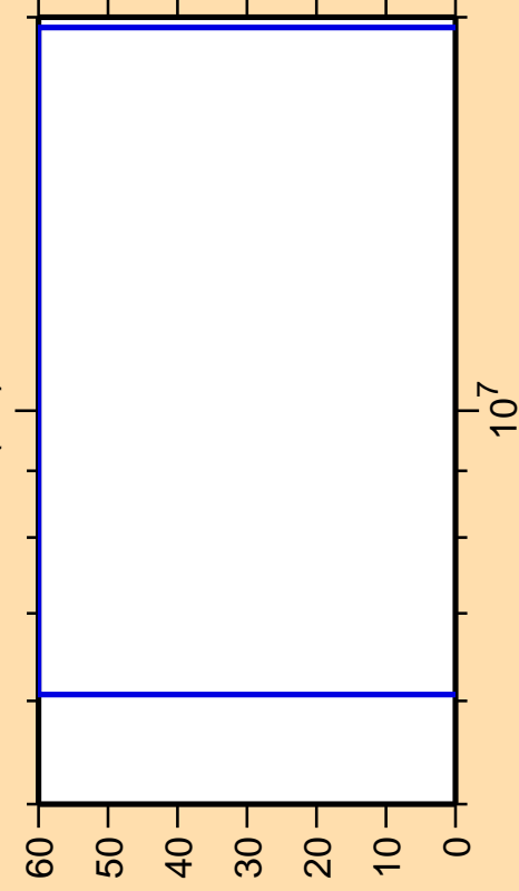
\Delta\sigma/\sigma vs. E for ^{99}\text{Pd}(n,t)
