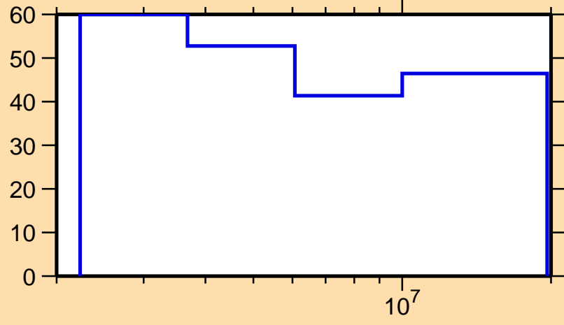
\Delta\sigma/\sigma vs. E for ^{99}\text{Pd}(n,ncont.)
