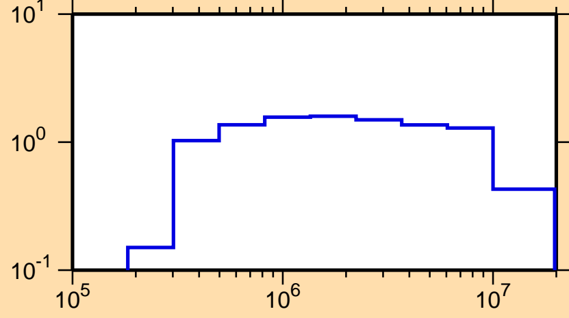
\sigma vs. E for ^{99}\text{Pd}(n,\text{inel.})
