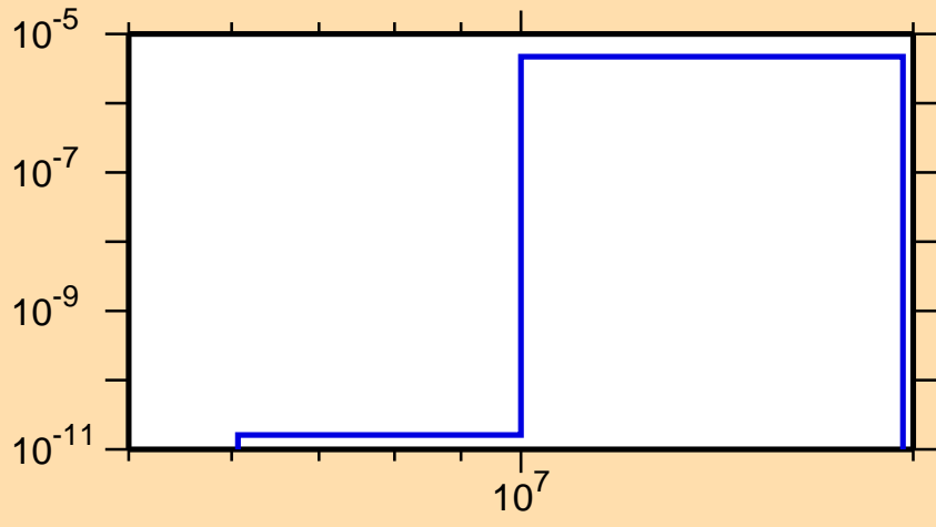
\sigma vs. E for ^{99}\text{Pd}(n,\text{He}3)
