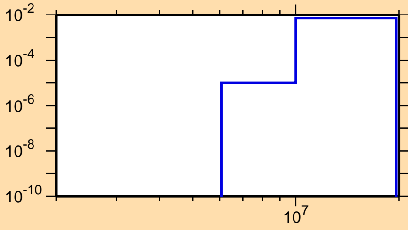
\sigma vs. E for ^{99}\text{Pd}(n,d)
