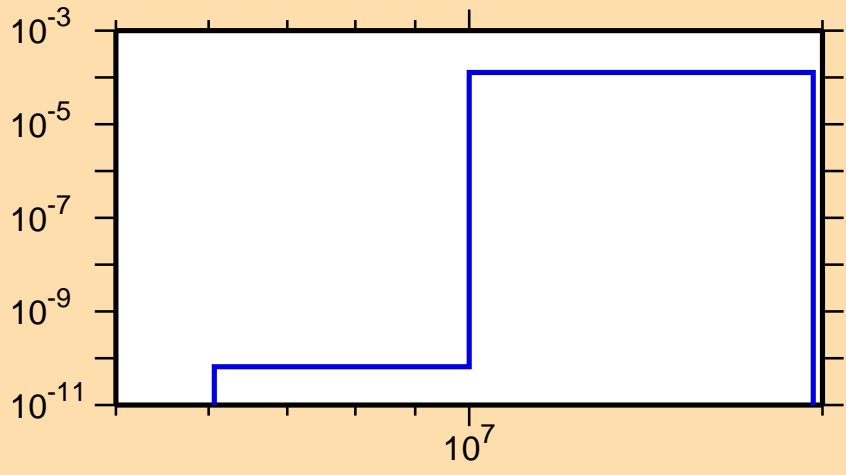
\sigma vs. E for ^{99}\text{Pd}(n,t)
