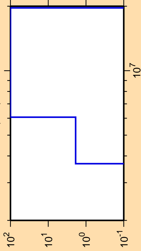
\Delta\sigma/\sigma vs. E for ^{99}\text{Pd}(n,d)
