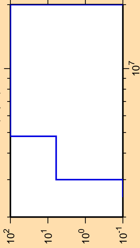
\Delta\sigma/\sigma vs. E for ^{99}\text{Pd}(n,p\alpha)
