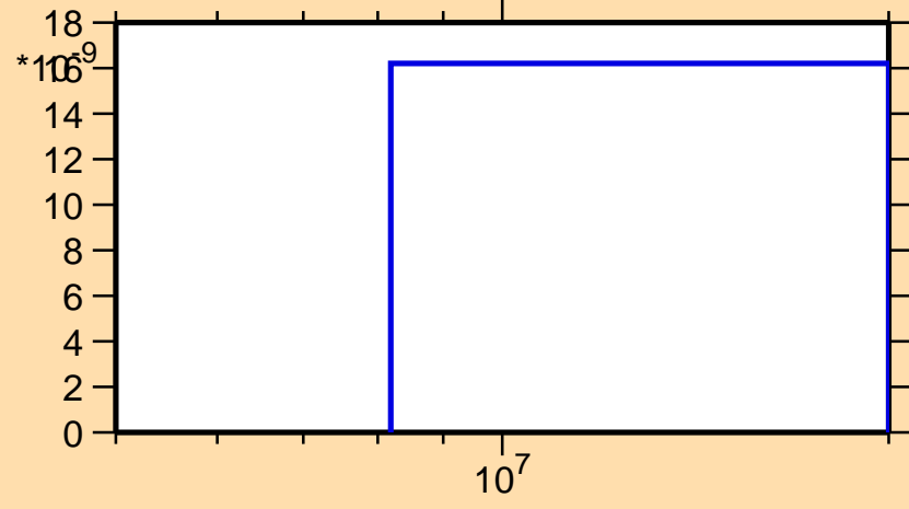
\sigma vs. E for ^{99}\text{Pd}(n,\text{pt})
