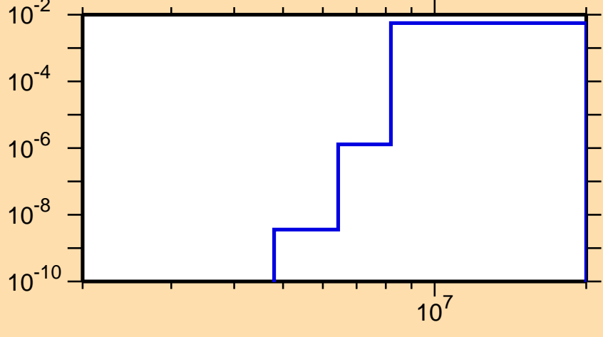
\sigma vs. E for ^{99}\text{Pd}(n,p\alpha)
