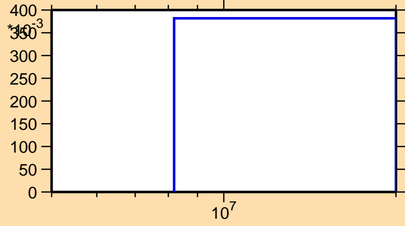
\sigma vs. E for ^{99}\text{Pd}(n,2n)
