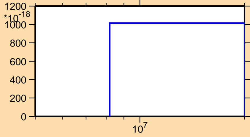
\sigma vs. E for ^{99}\text{Pd}(n,nt)
