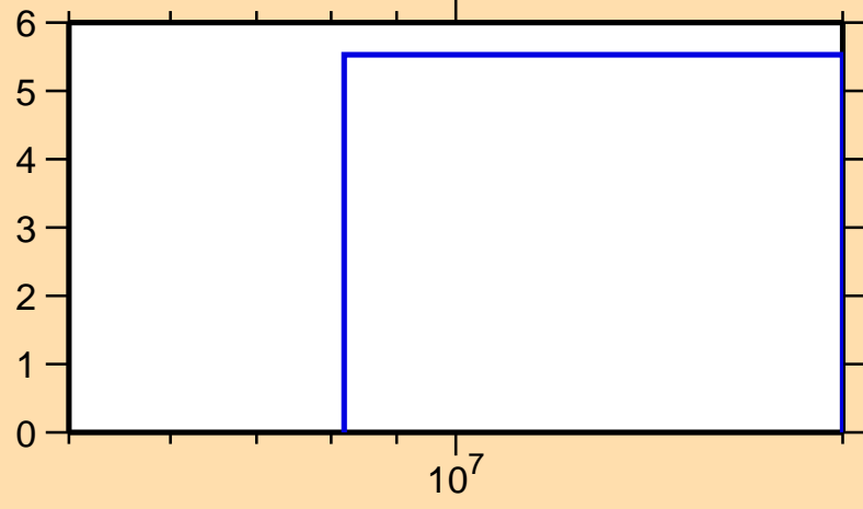
\Delta\sigma/\sigma vs. E for ^{99}\text{Pd}(n,\text{nonel.})
