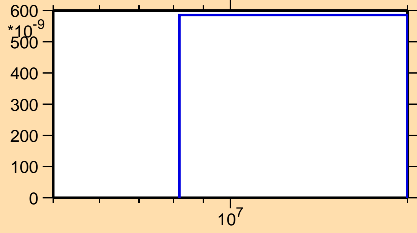
\sigma vs. E for ^{99}\text{Pd}(n,\text{nd})
