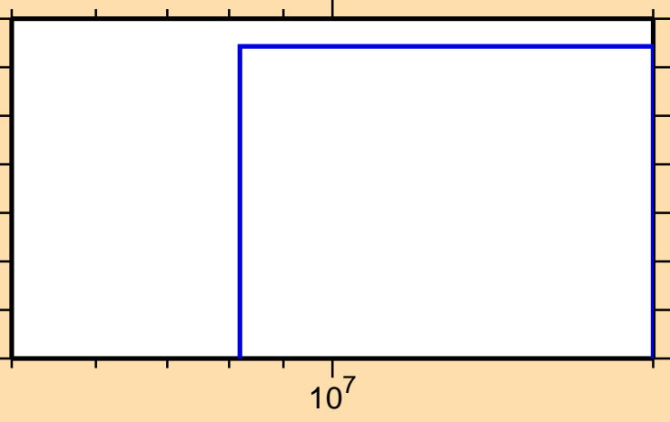
\sigma vs. E for ^{99}\text{Pd}(\text{mt117})
