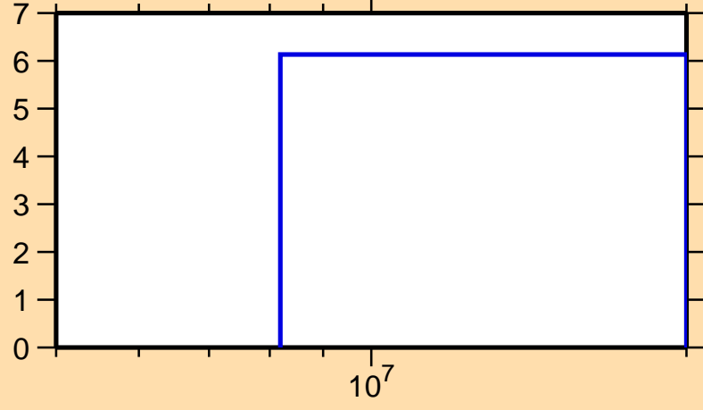
\Delta\sigma/\sigma vs. E for ^{99}\text{Pd}(n,\text{tot.})
