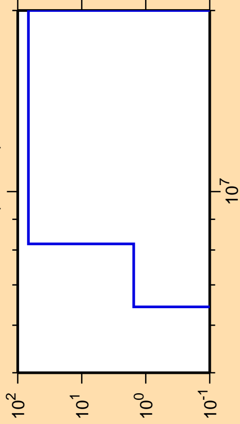
\Delta\sigma/\sigma vs. E for ^{99}\text{Pd}(n,\text{He}3)
