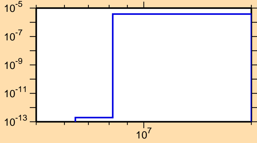
\sigma vs. E for ^{99}\text{Pd}(n,\text{He}3)
