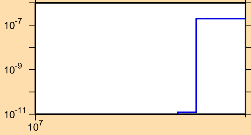
\sigma vs. E for ^{100}\text{Pd}(n,2n\alpha)
