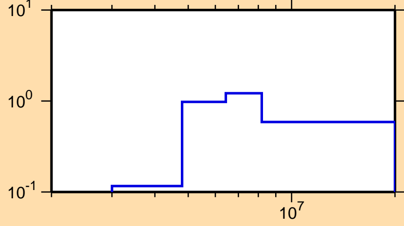
\sigma vs. E for ^{100}\text{Pd}(n,n\text{cont.})
