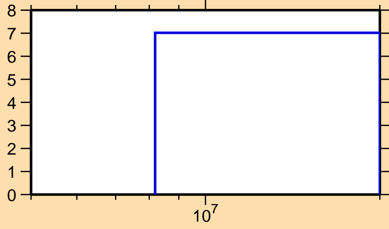
\Delta\sigma/\sigma vs. E for ^{100}\text{Pd}(n,\text{nonel.})
