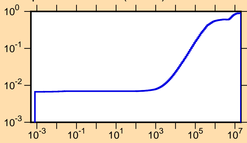
\mu vs. E for ^{101}\text{Pd}(\text{mt251})
