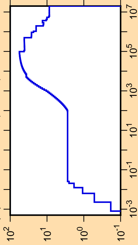
\Delta\mu/\mu vs. E for ^{101}\text{Pd}(\text{mt251})
