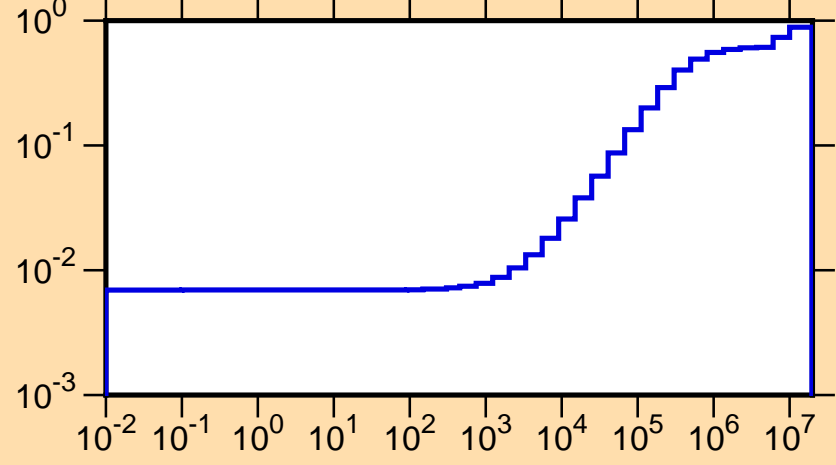
\mu vs. E for ^{101}\text{Pd}(\text{mt251})
