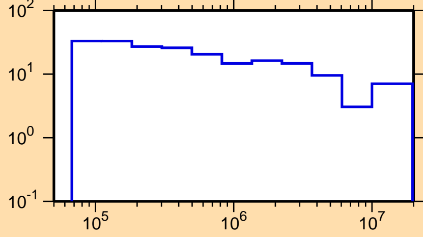
\Delta\sigma/\sigma vs. E for ^{101}\text{Pd}(n,\text{tot.})
