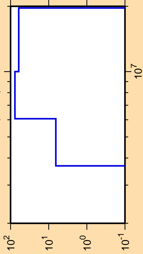
\Delta\sigma/\sigma vs. E for ^{101}\text{Pd}(n,n\alpha)
