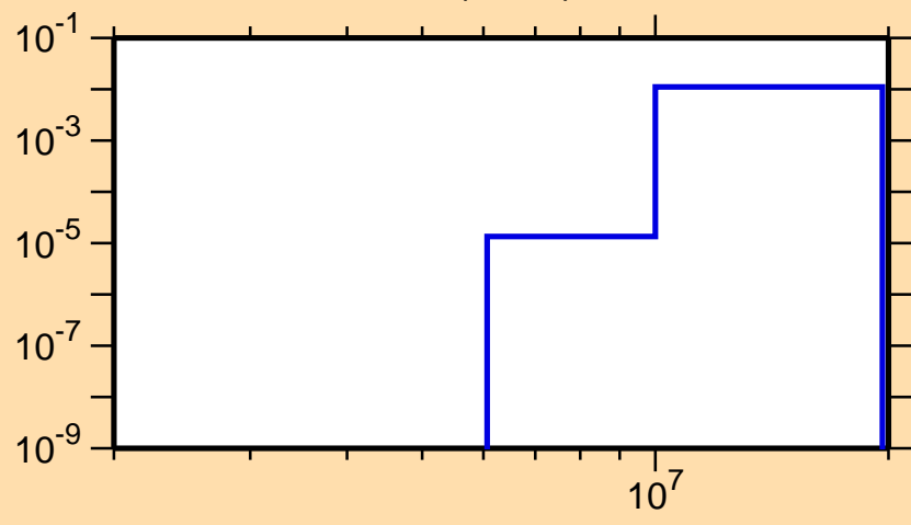
\sigma vs. E for ^{101}\text{Pd}(n,n\alpha)
