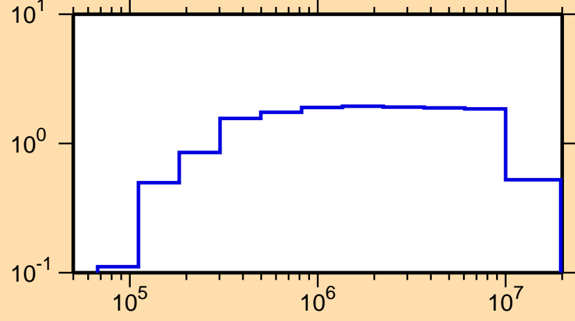
\sigma vs. E for ^{101}\text{Pd}(n,\text{inel.})
