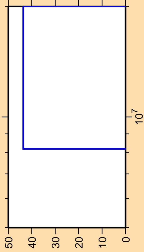
\Delta\sigma/\sigma vs. E for ^{101}\text{Pd}(n,p)
