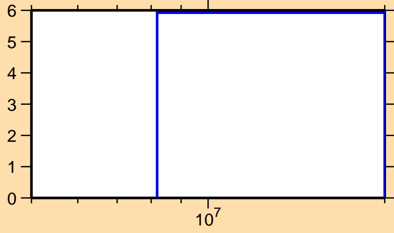
\Delta\sigma/\sigma vs. E for ^{101}\text{Pd}(n,\text{tot.})
