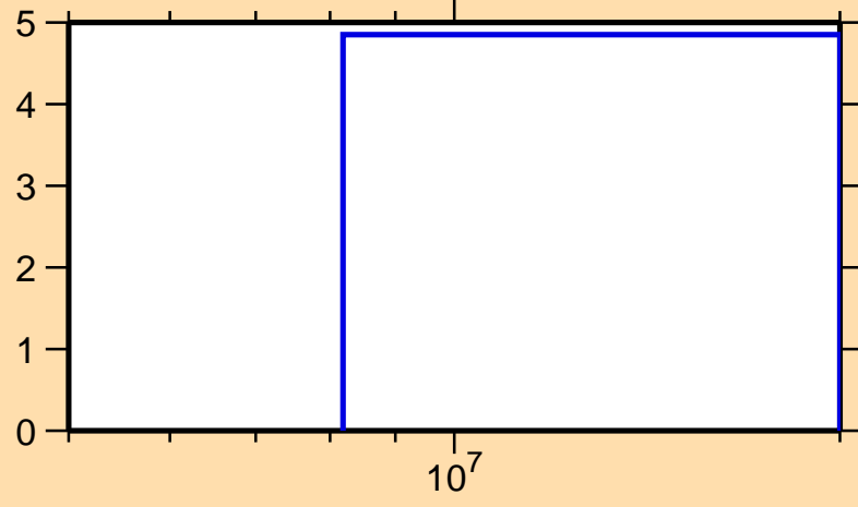
\Delta\sigma/\sigma vs. E for ^{101}\text{Pd}(n,\text{nonel.})
