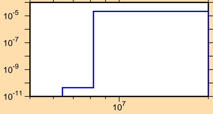
\sigma vs. E for ^{101}\text{Pd}(n,p\alpha)
