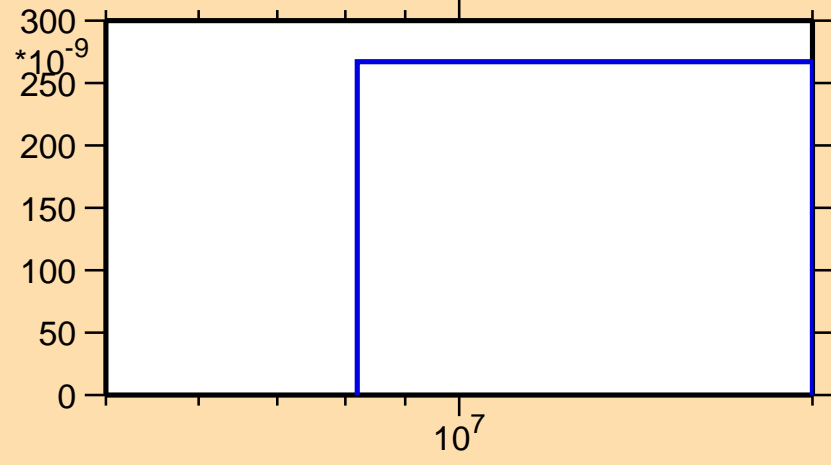
\sigma vs. E for ^{101}\text{Pd}(n,\text{He3})
