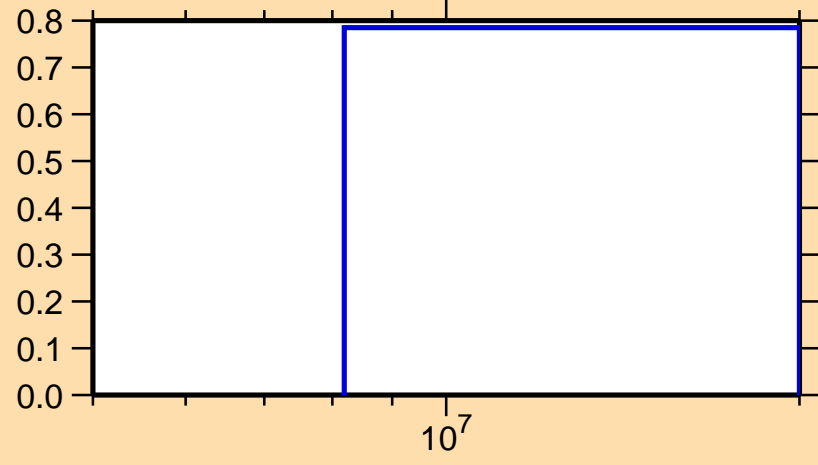
\sigma vs. E for ^{101}\text{Pd}(n,2n)
