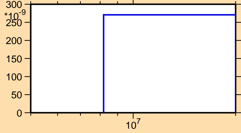
\sigma vs. E for ^{101}\text{Pd}(n,2n\alpha)
