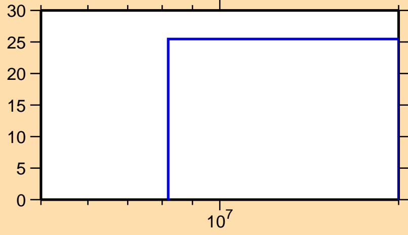
\Delta\sigma/\sigma vs. E for ^{101}\text{Pd}(n,\text{inel.})
