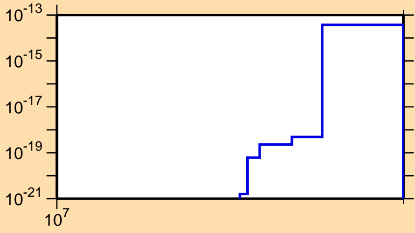
\sigma vs. E for ^{102}\text{Pd}(n,\text{pt})
