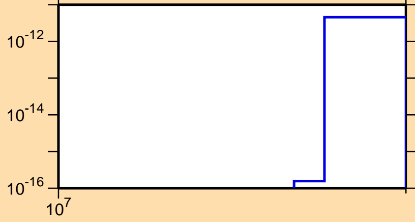
\sigma vs. E for ^{102}\text{Pd}(\text{mt } 45)
