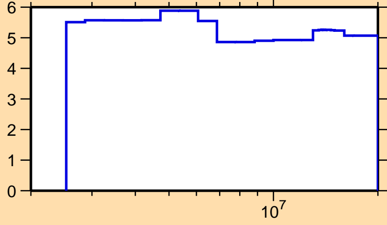
\Delta\sigma/\sigma vs. E for ^{102}\text{Pd}(n,n\text{nonel.})
