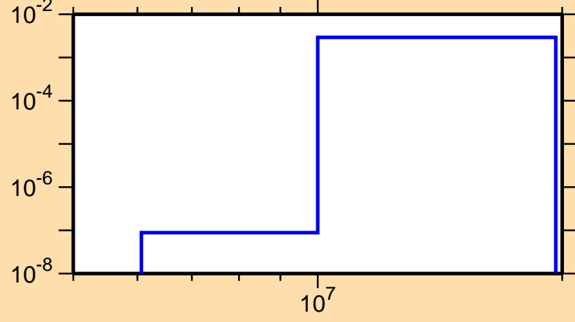
\sigma vs. E for ^{102}\text{Pd}(n,d)
