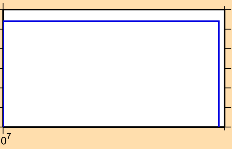
\sigma vs. E for ^{102}\text{Pd}(n,3n)
