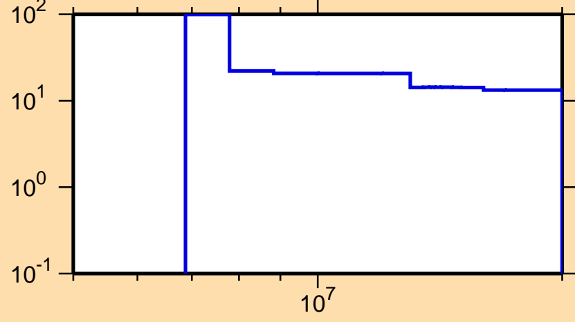
\Delta\sigma/\sigma vs. E for ^{103}\text{Pd}(n,2n)
