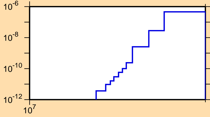
\sigma vs. E for ^{103}\text{Pd}(n,\text{He}3)
