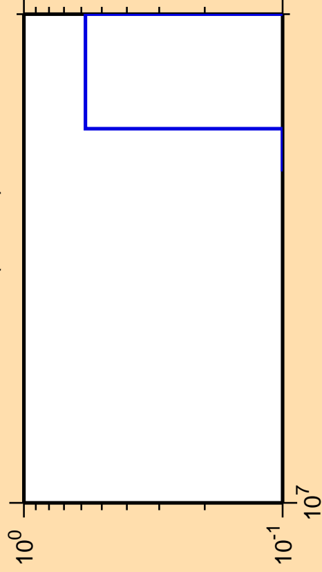
\Delta\sigma/\sigma vs. E for ^{103}\text{Pd}(\text{mt } 45)
