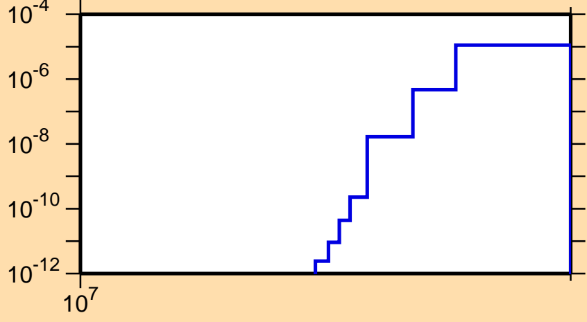
\sigma vs. E for ^{103}\text{Pd}(n,2n\alpha)
