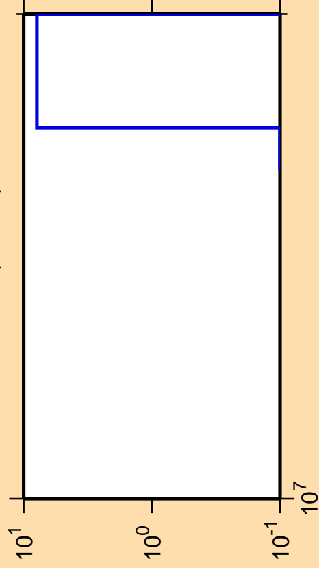
\Delta\sigma/\sigma vs. E for ^{103}\text{Pd}(\text{mt } 34)
