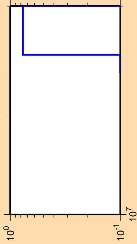
\Delta\sigma/\sigma vs. E for ^{103}\text{Pd}(\text{mt117})
