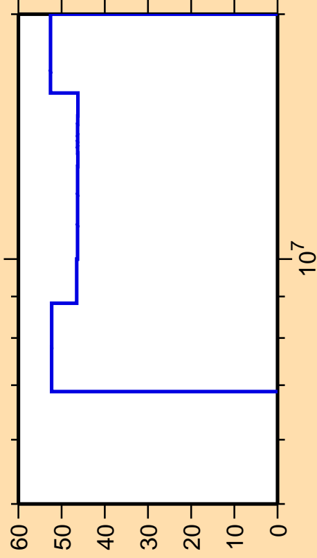
\Delta\sigma/\sigma vs. E for ^{103}\text{Pd}(n,p)
