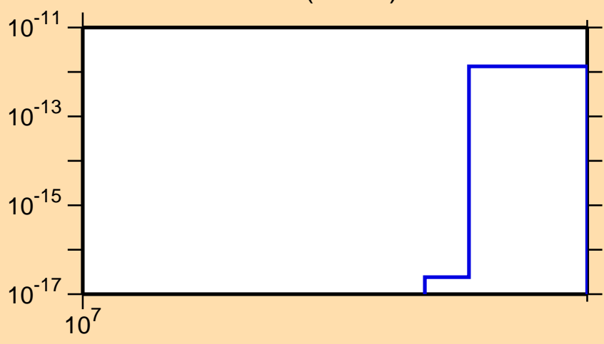
\sigma vs. E for ^{103}\text{Pd}(\text{mt } 34)
