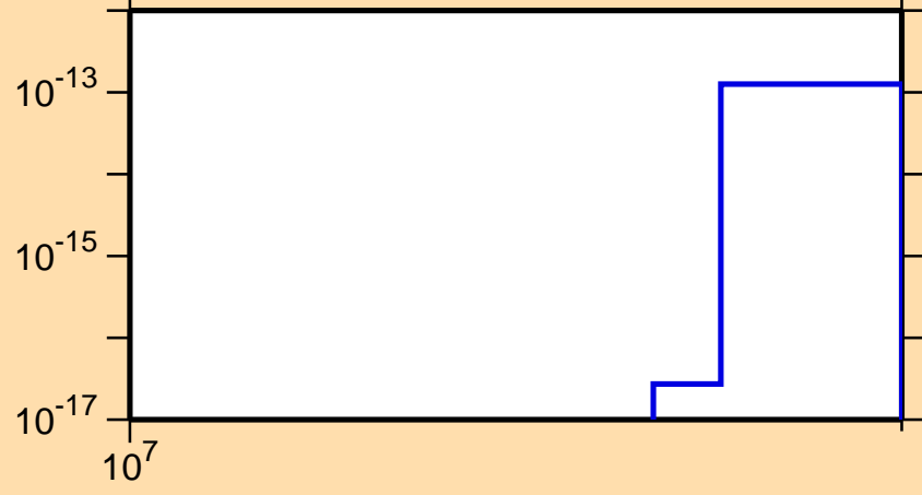
\sigma vs. E for ^{103}\text{Pd}(\text{mt } 45)
