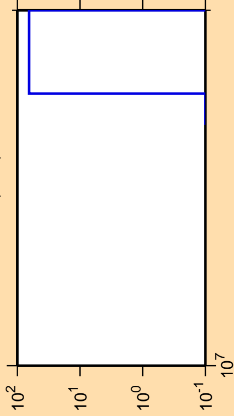
\Delta\sigma/\sigma vs. E for ^{103}\text{Pd}(n,nt)
