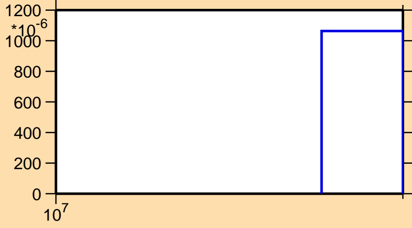
\sigma vs. E for ^{103}\text{Pd}(n,3n)
