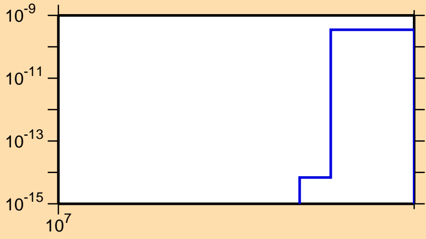
\sigma vs. E for ^{103}\text{Pd}(n,\text{pt})
