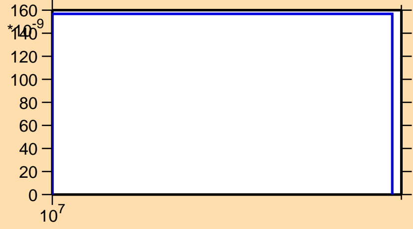
\sigma vs. E for ^{103}\text{Pd}(n,\text{nd})
