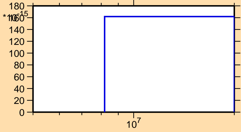
\sigma vs. E for ^{103}\text{Pd}(n,\text{nt})
