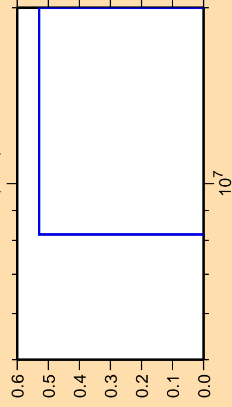
\Delta\sigma/\sigma vs. E for ^{103}\text{Pd}(n,\text{nt})
