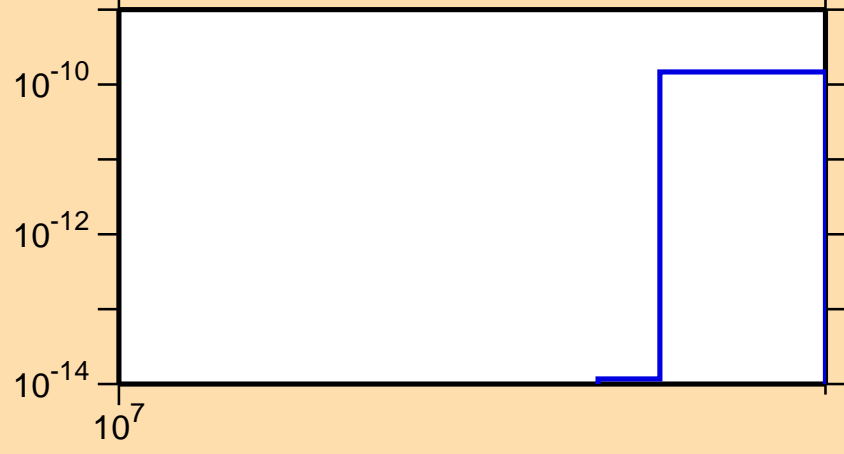
\sigma vs. E for ^{104}\text{Pd}(n,\text{pd})
