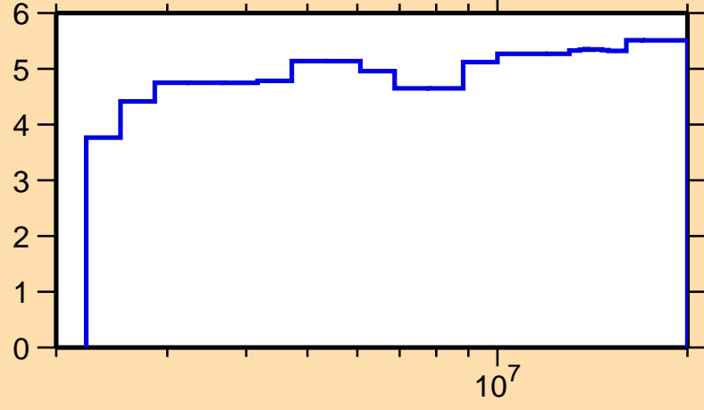
\Delta\sigma/\sigma vs. E for ^{104}\text{Pd}(n,n\text{onel.})
