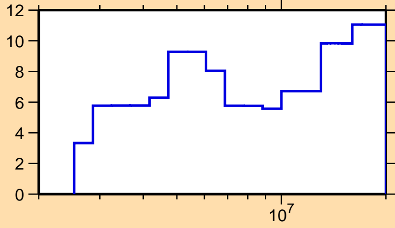
\Delta\sigma/\sigma vs. E for ^{104}\text{Pd}(n,el.)
