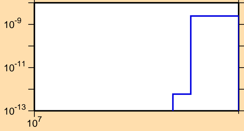
\sigma vs. E for ^{104}\text{Pd}(n,2n\alpha)
