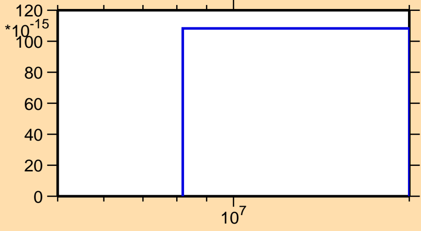
\sigma vs. E for ^{104}\text{Pd}(n,\text{nt})
