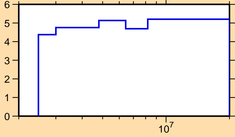
\Delta\sigma/\sigma vs. E for ^{104}\text{Pd}(n,n\text{nonel.})
