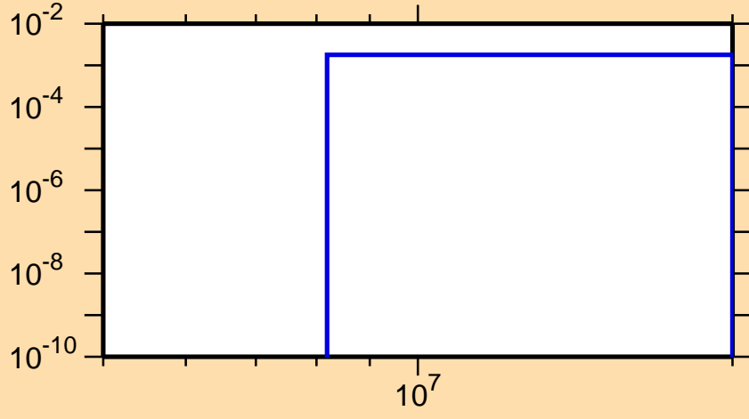
\sigma vs. E for ^{104}\text{Pd}(n,d)
