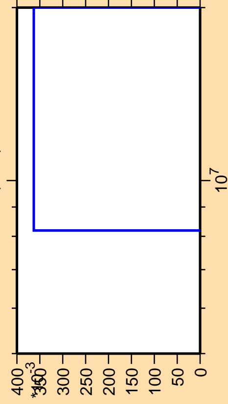
\Delta\sigma/\sigma vs. E for ^{104}\text{Pd}(n,\text{nt})
