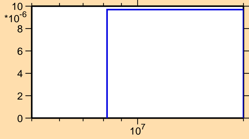
\sigma vs. E for ^{104}\text{Pd}(n,t)
