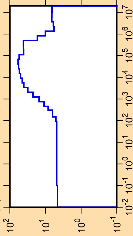
\Delta\mu/\mu vs. E for ^{105}\text{Pd}(\text{mt251})
