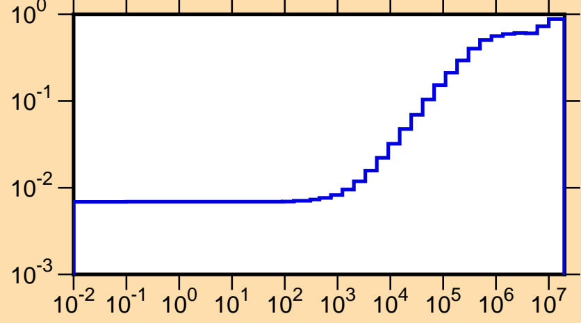
\mu vs. E for ^{105}\text{Pd}(\text{mt251})
